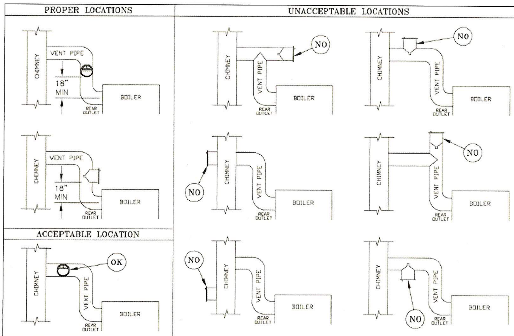
Figure 19: Proper and Improper Locations of Draft Regulator
