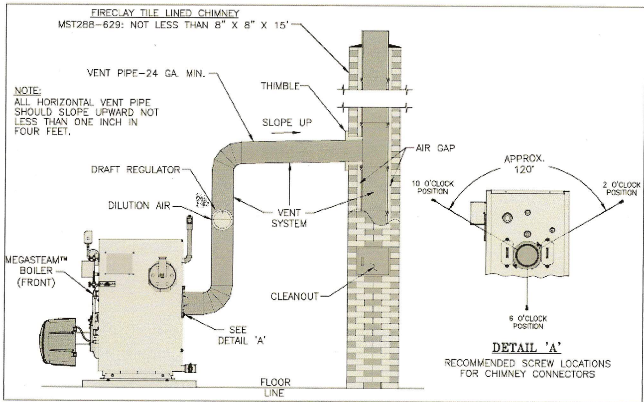
Figure 18: Recommended Vent Pipe Arrangement and Chimney Requirements
