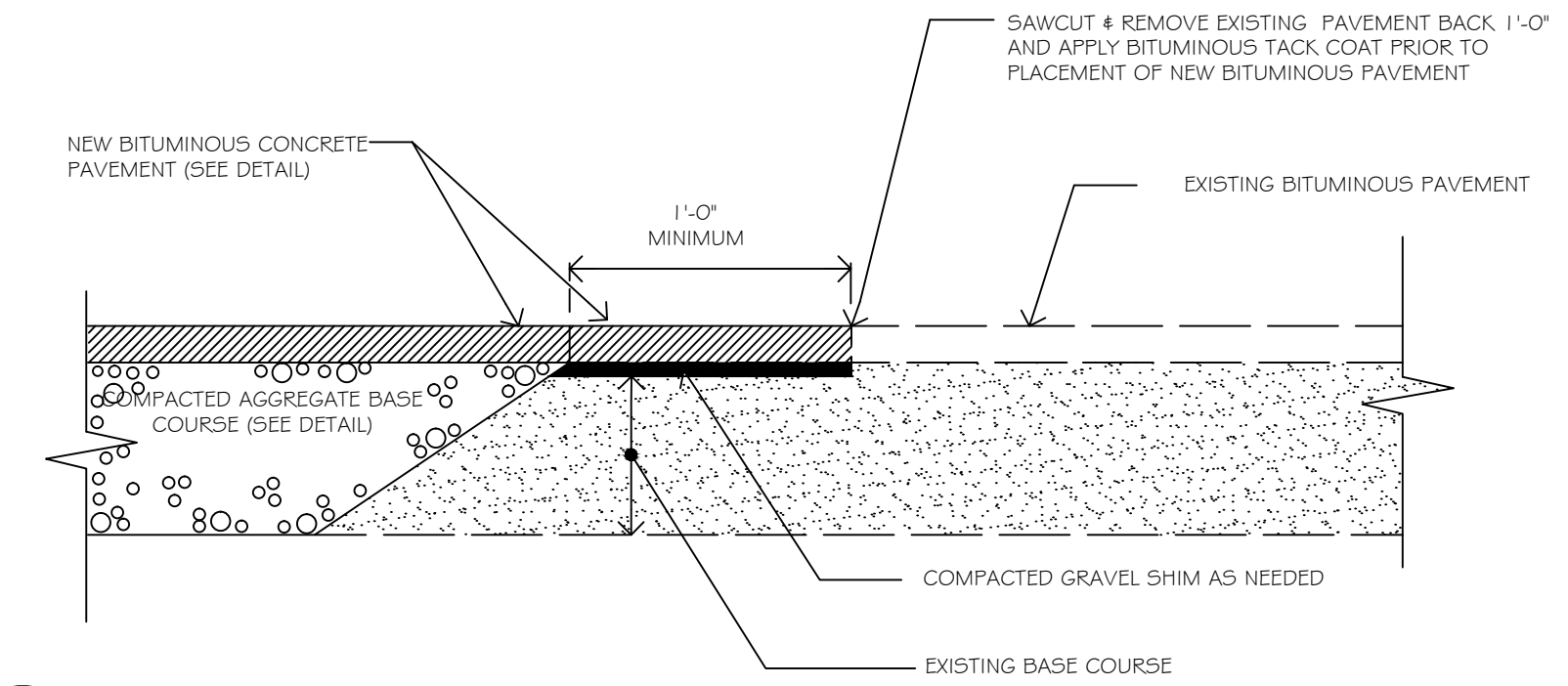
3 PAVEMENT SAW CUT DETAIL C3.1 NOT TO SCALE
