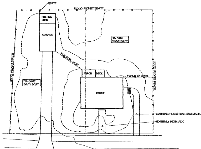
1 SITE PLAN A001 SCALE: 1/16"=1'-0"
