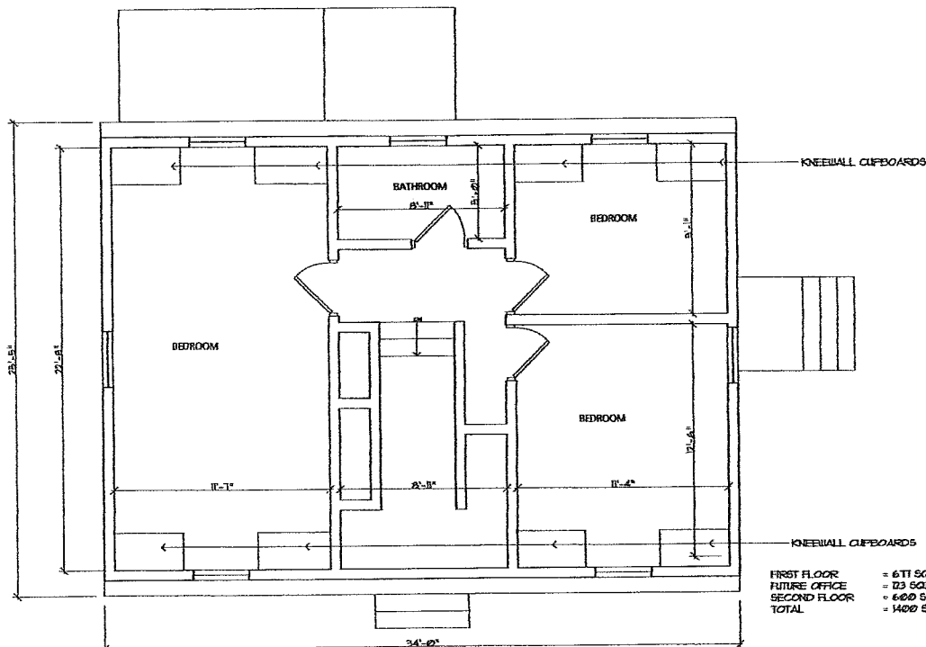
1 SECOND FLOOR PLAN A002 SCALE: 1/4" = 1'-0"
