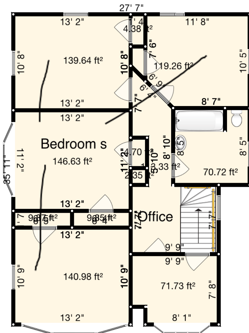
Existing second floor
