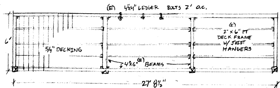
A2 1 PORCH DECK FRAMING DETAIL SCALE 1/4" PER FOOT
