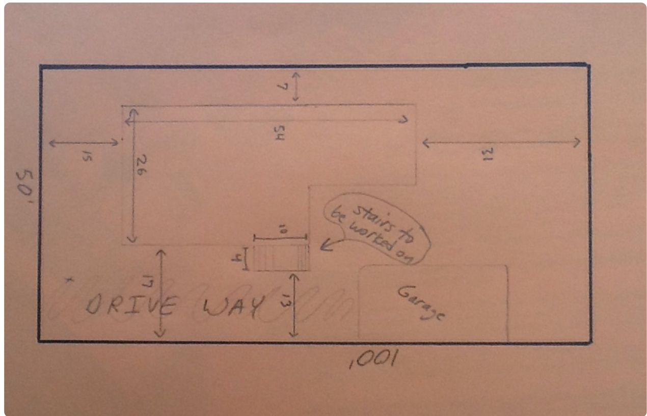
51 Hillis plot
