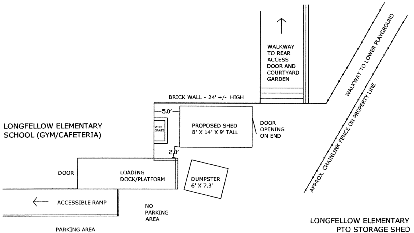
LOCATION PLAN
