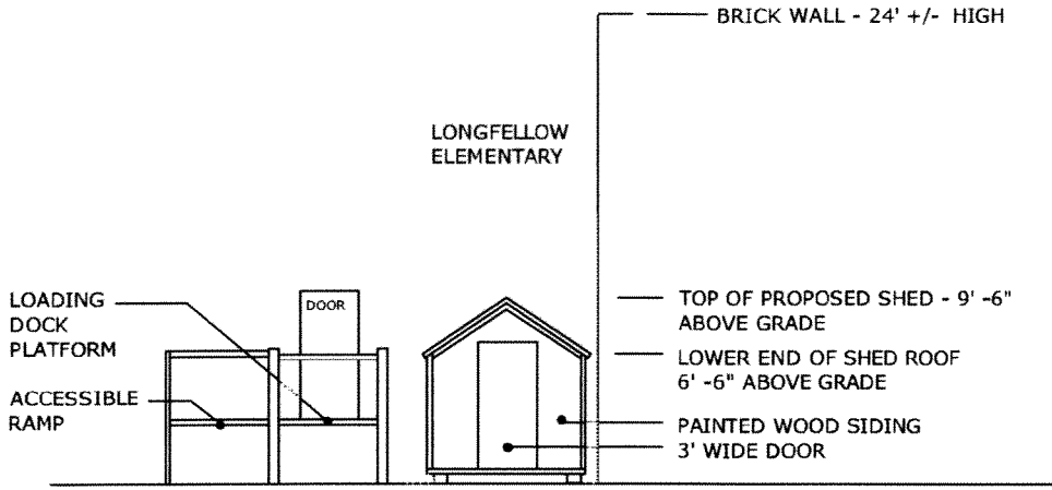
ELEVATION VIEW
