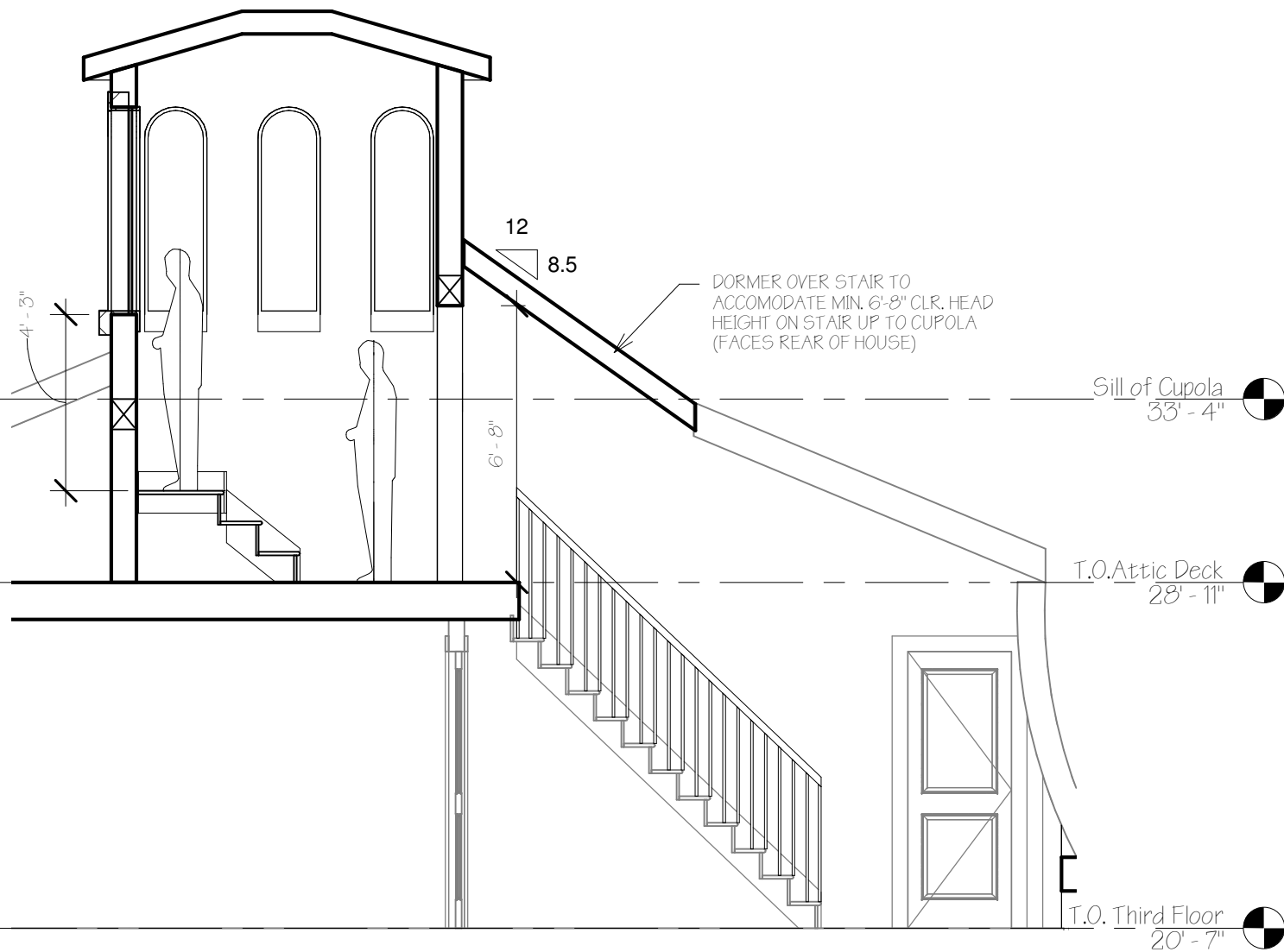
E Section Showing Observation Platform 1/4" = 1'-0"
