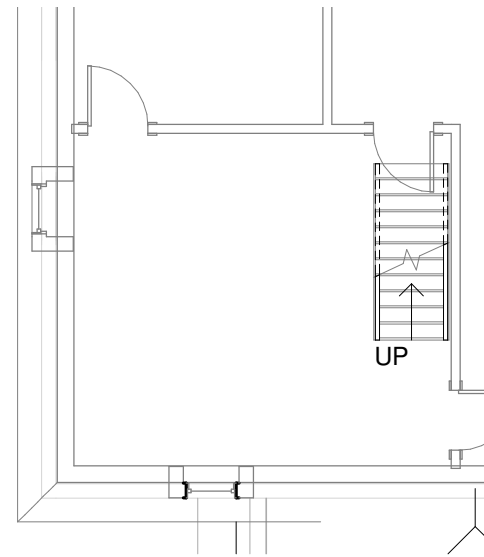
B Third Floor 1/8" = 1'-0"
