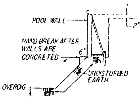
FIGURE 2 -- INITIAL FORMING OF POOL BOTTOM
