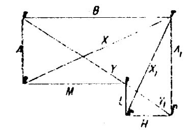
1C -- TRUE "L" STAKEOUT
