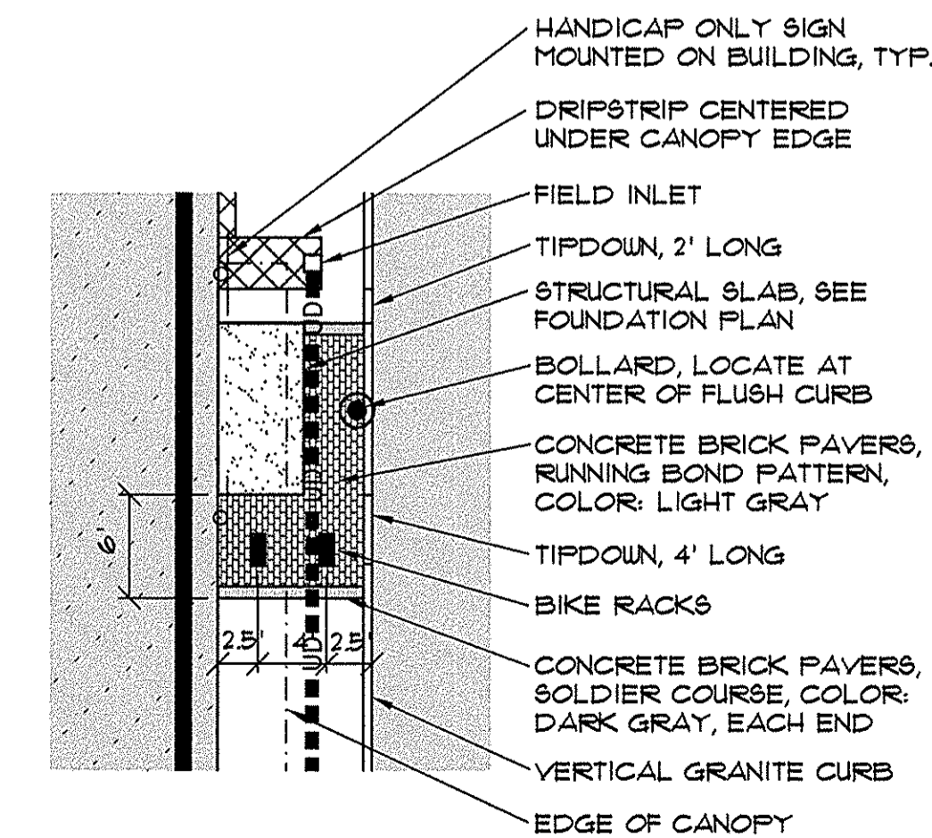
SIDE ENTRANCE DETAIL
