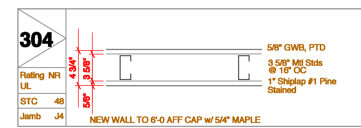
Gypsum Partition at Conf Room
