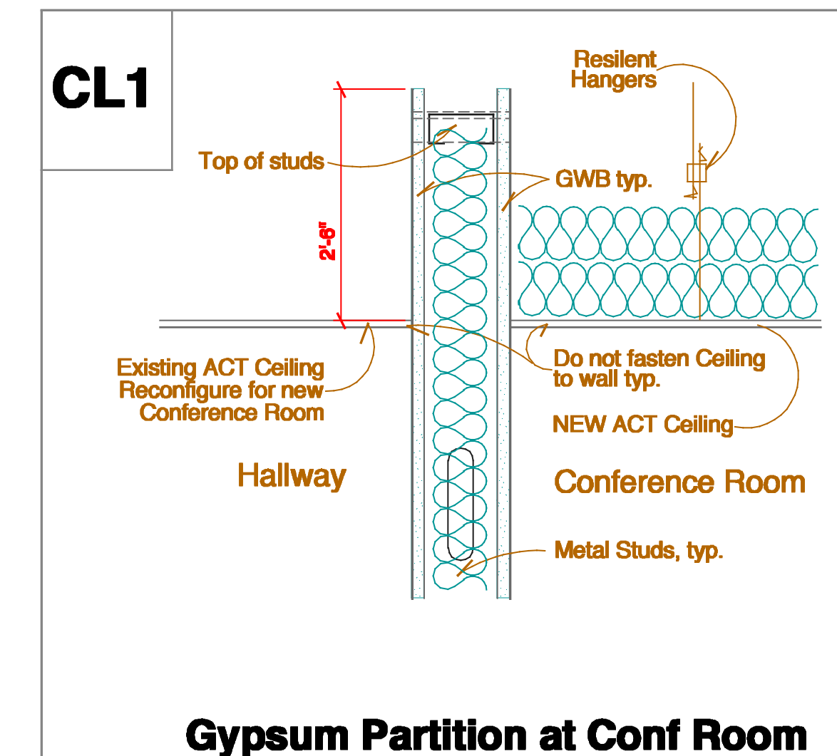
Typ Gypsum Partition at Offices
