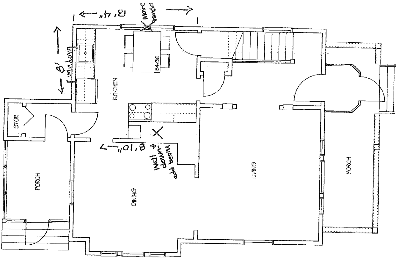
First Floor
