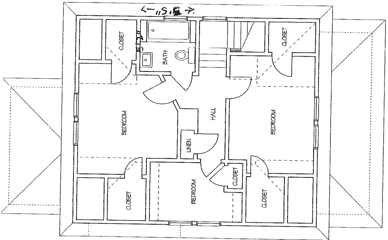
Second Floor
