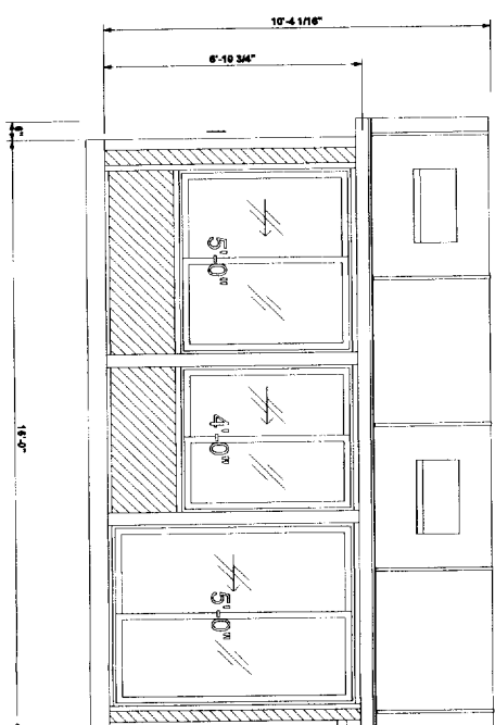
Front Elevation
