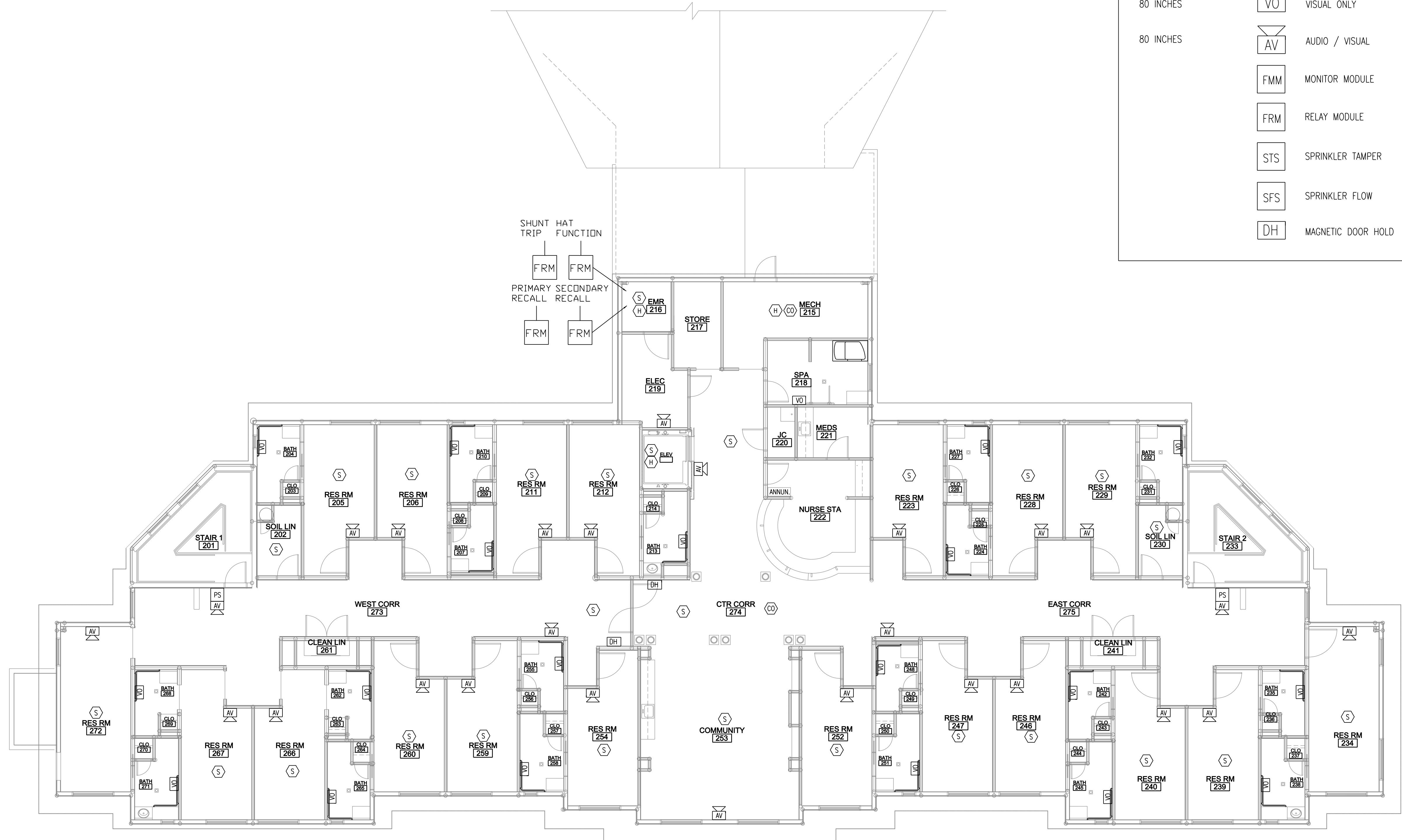
2ND FLOOR FIRE ALARM PLAN SCALE: 1/8" = 1'-0"
