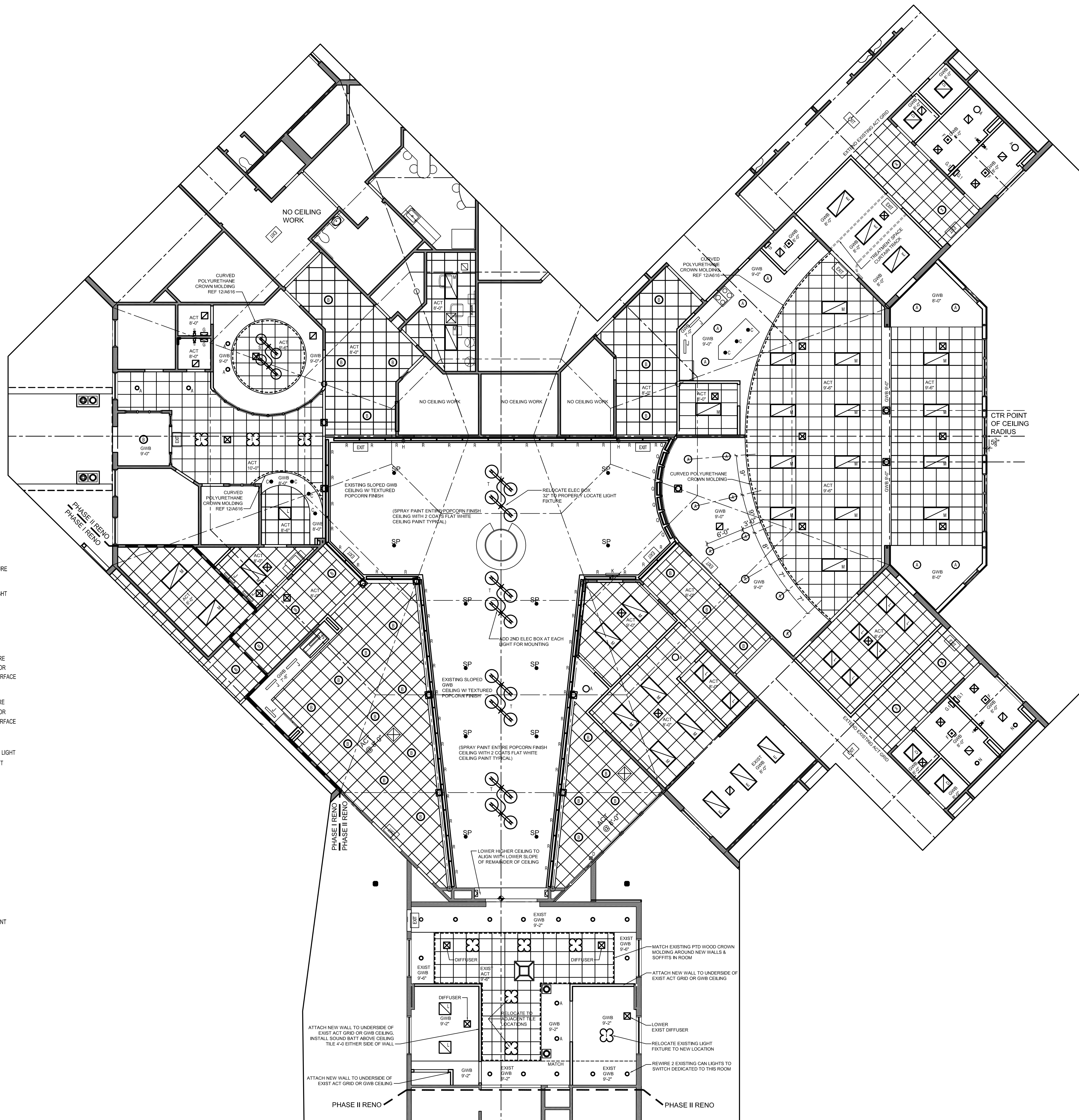
1 REFLECTED CEILING PLAN SCALE: 1/8" = 1'-0"
