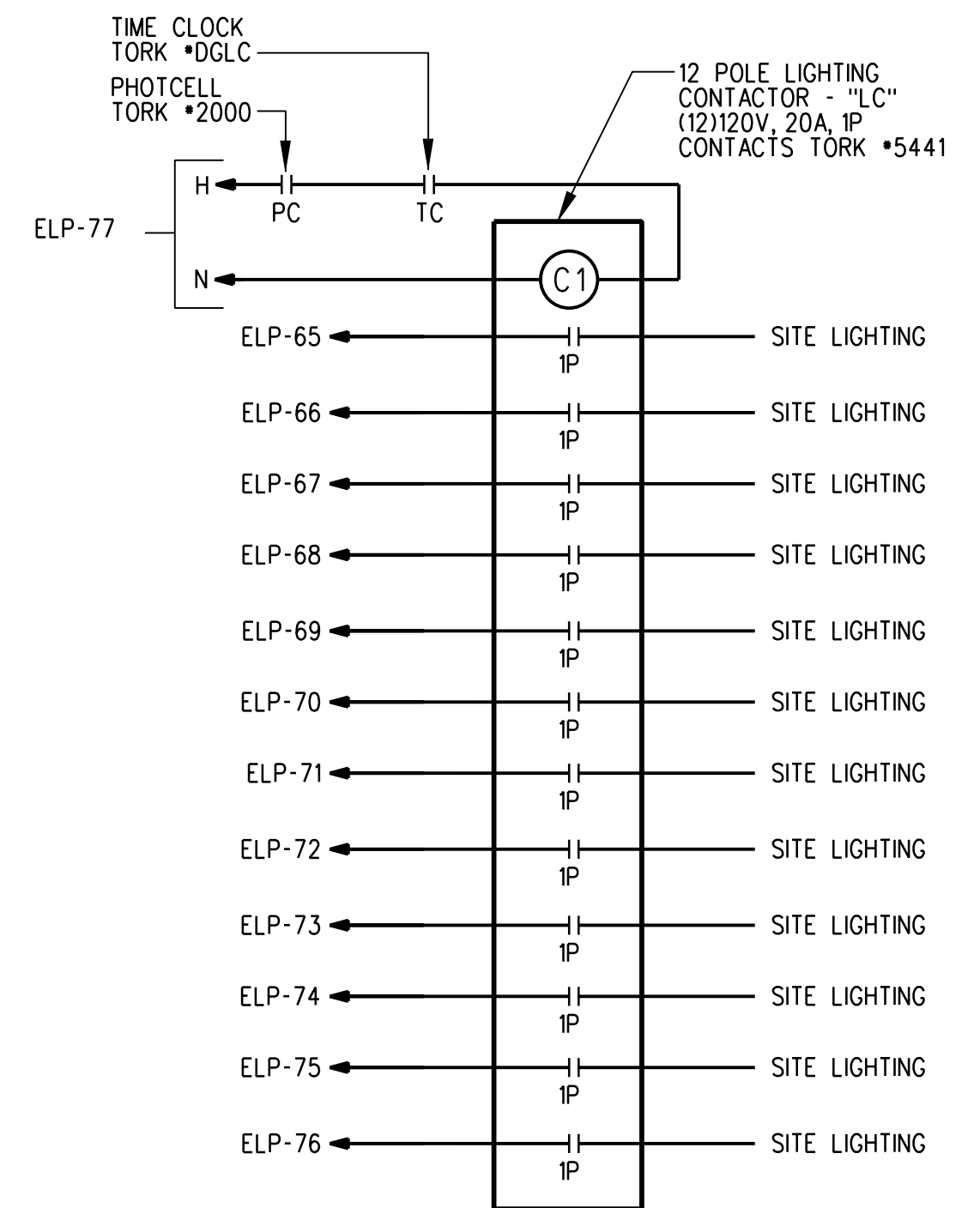
LIGHTING CONTACTOR "LC" DETAIL (EXTERIOR LIGHTING) SCALE: NONE
