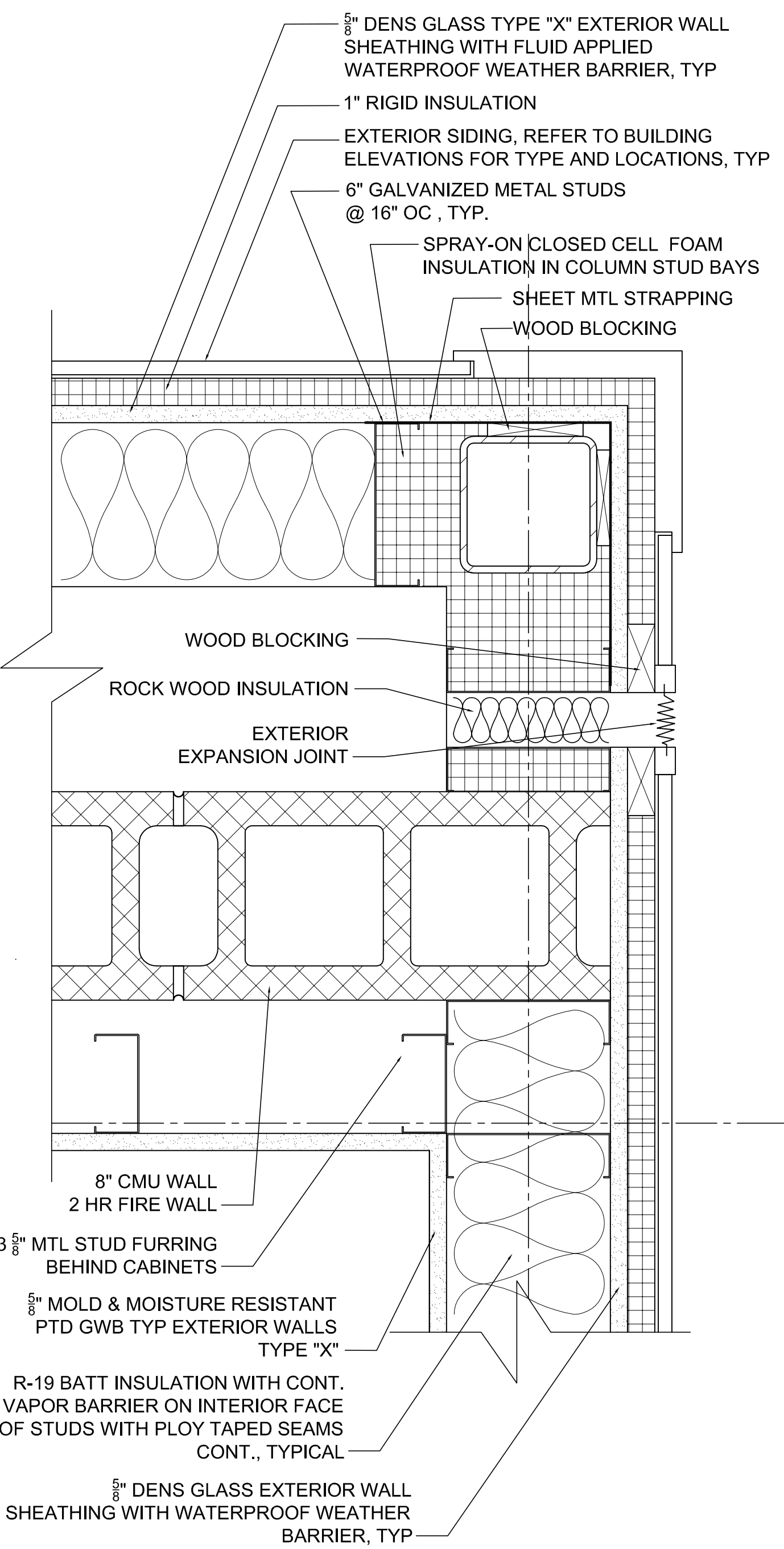
9 EXT COL / EXP JOINT DETAIL SCALE: 3" = 1'-0"
