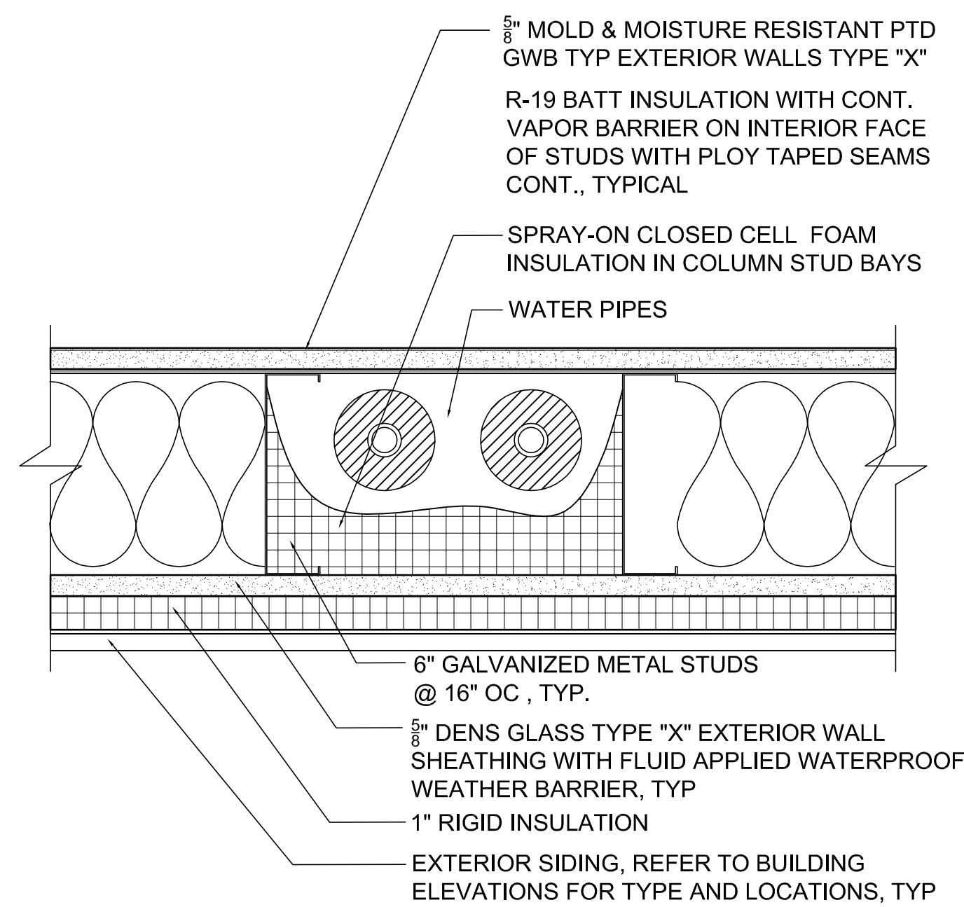
2 EXTERIOR WALL PIPE CHASE SCALE: 3" = 1'-0"
