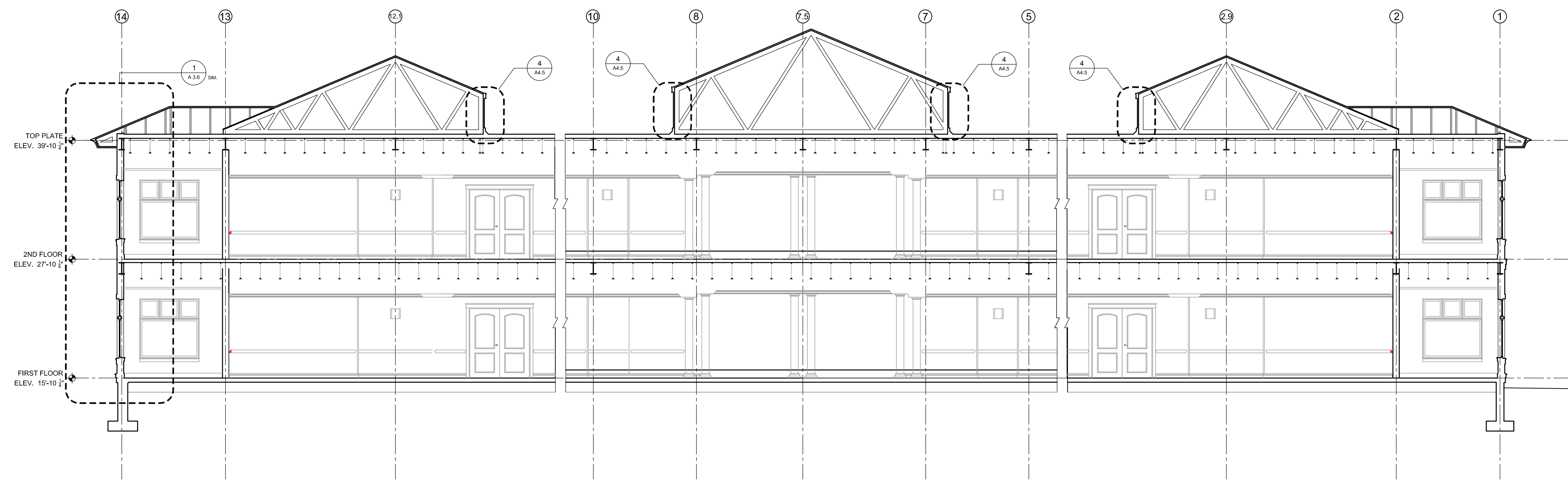
2 BUILDING SECTION SCALE: 3/16" = 1'-0"
