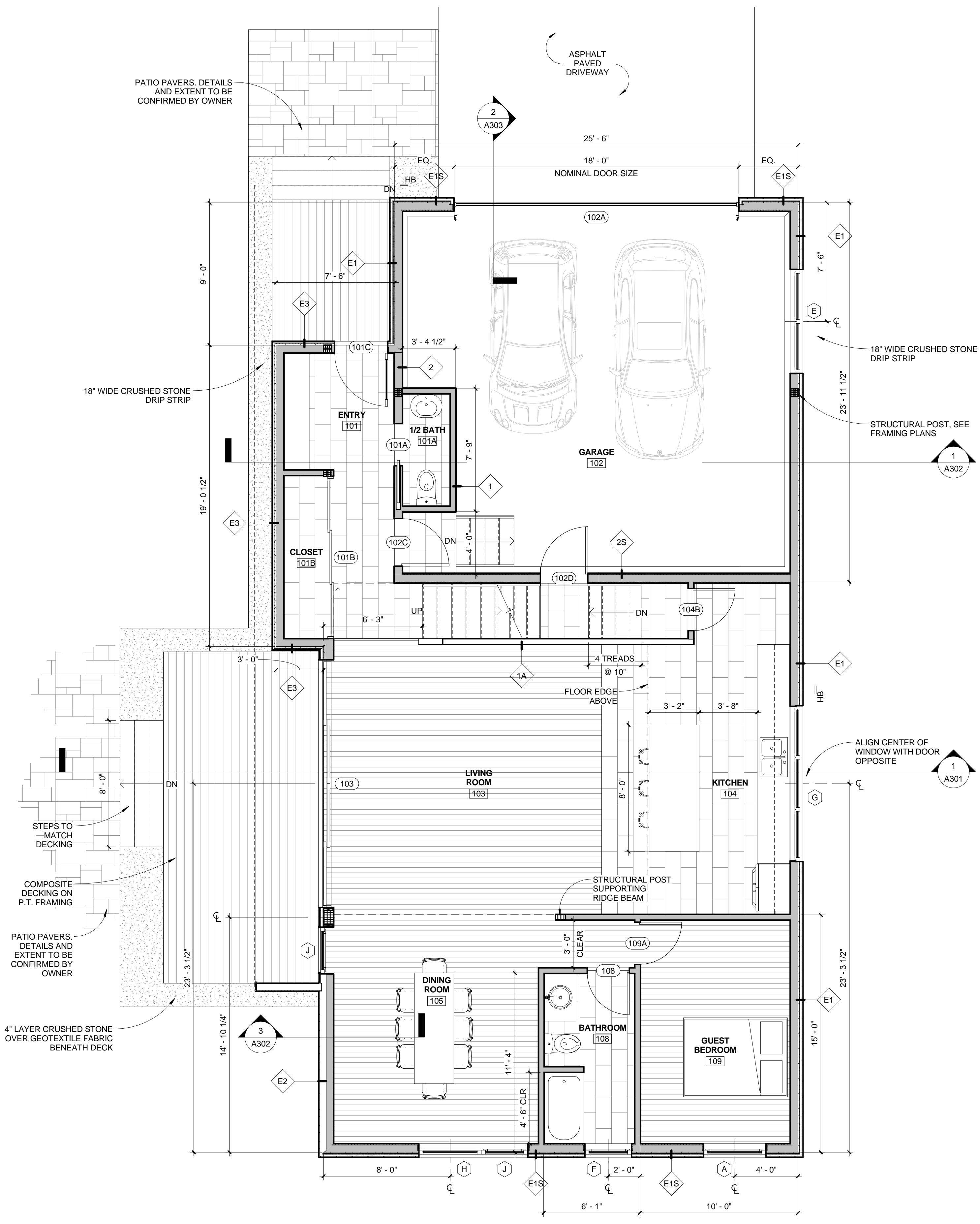
1 FIRST FLOOR PLAN 1/4" = 1'-0"
