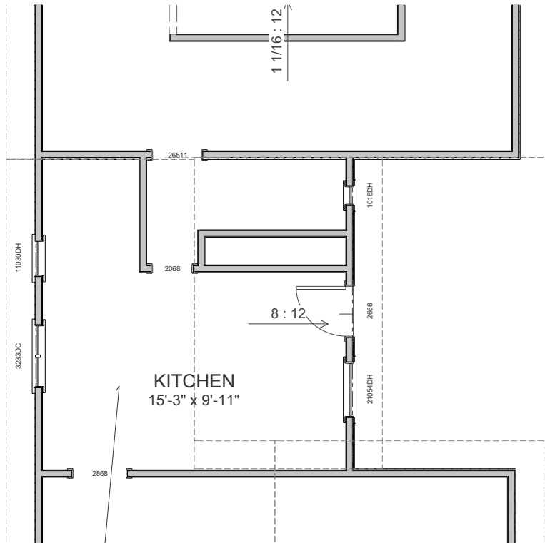
2nd Floor
