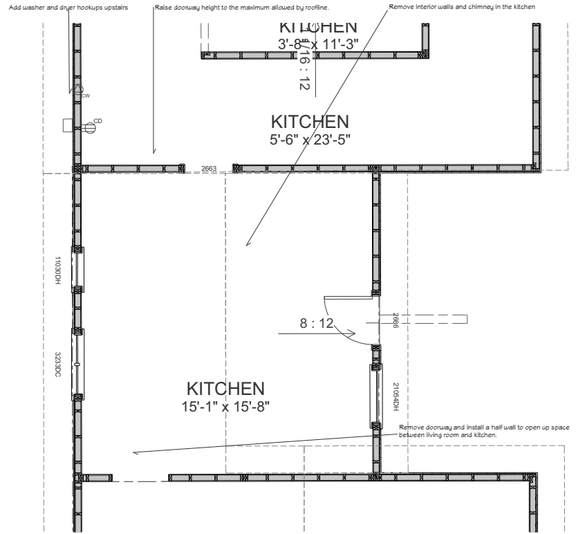
2nd Floor
