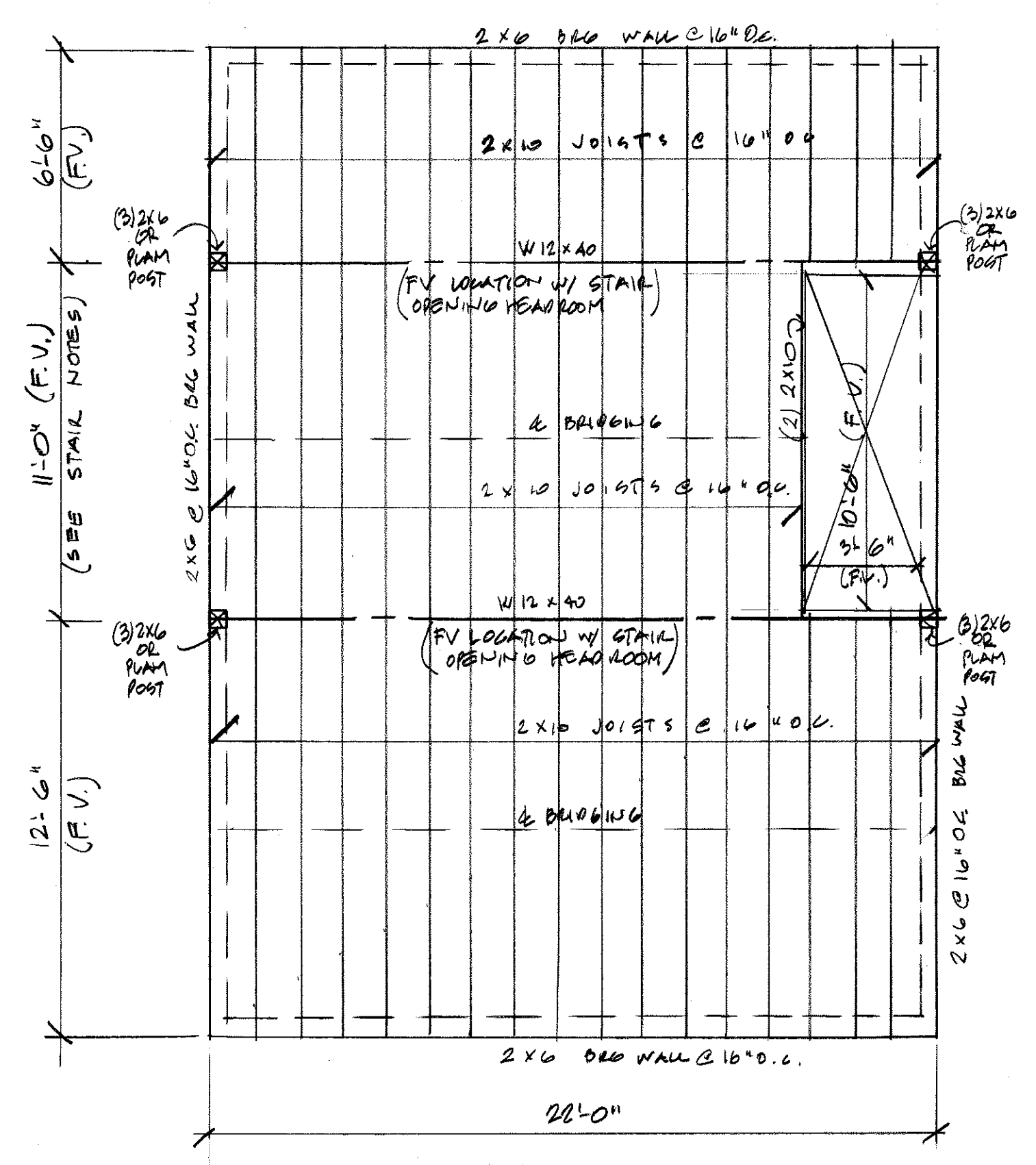
SECOND FLOOR FRAMING PLAN 1/4" = 1'-0"
