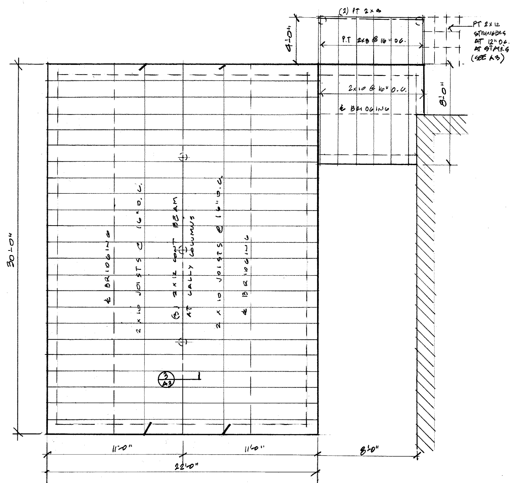
FIRST FLOOR FRAMING PLAN 1/4" = 1'-0"
