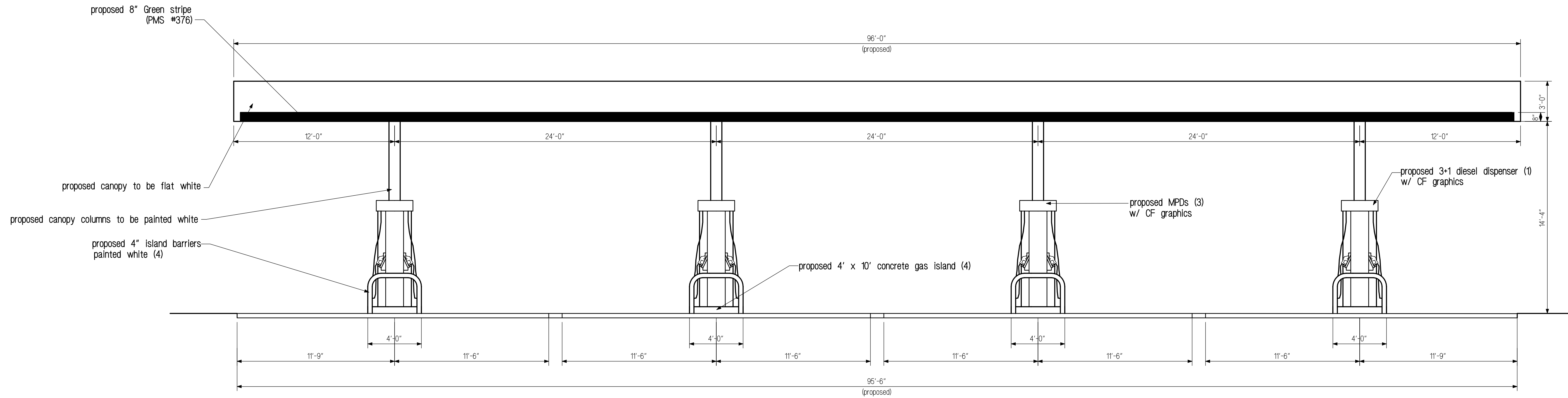
FRONT VIEW
