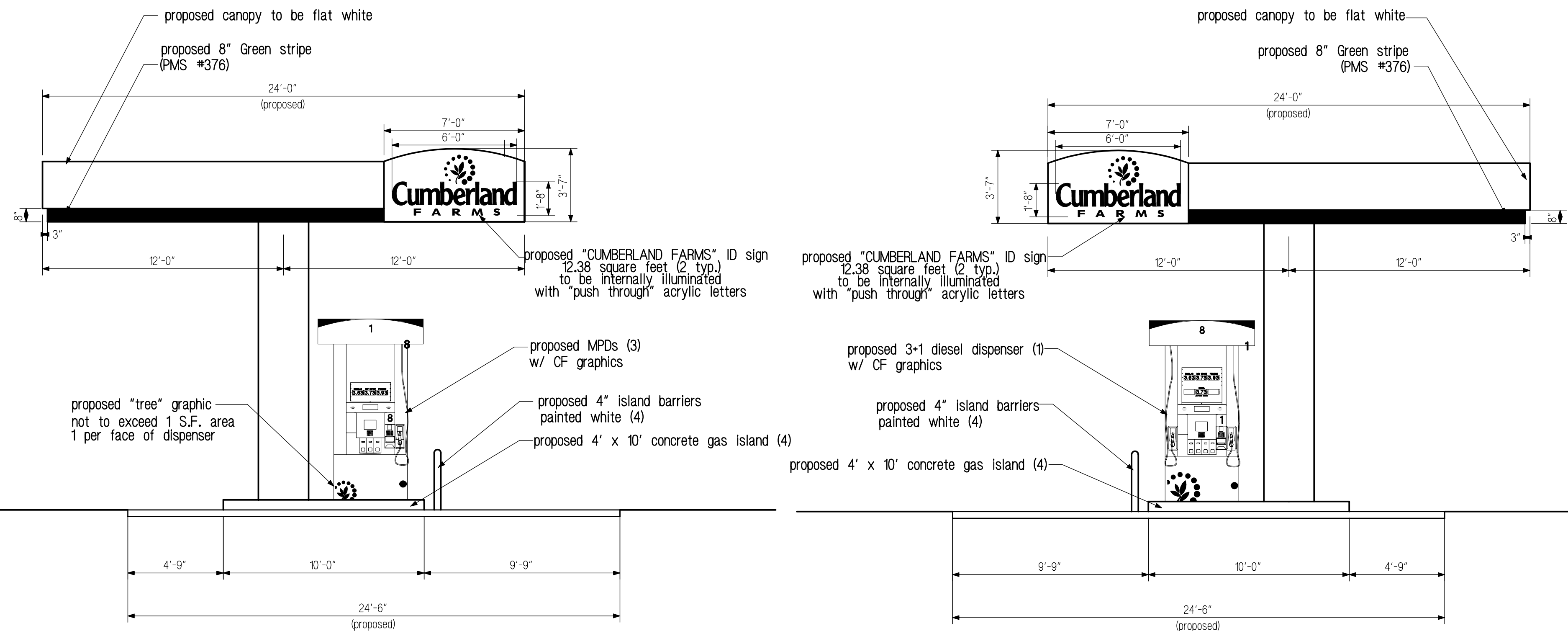
LEFT VIEW
