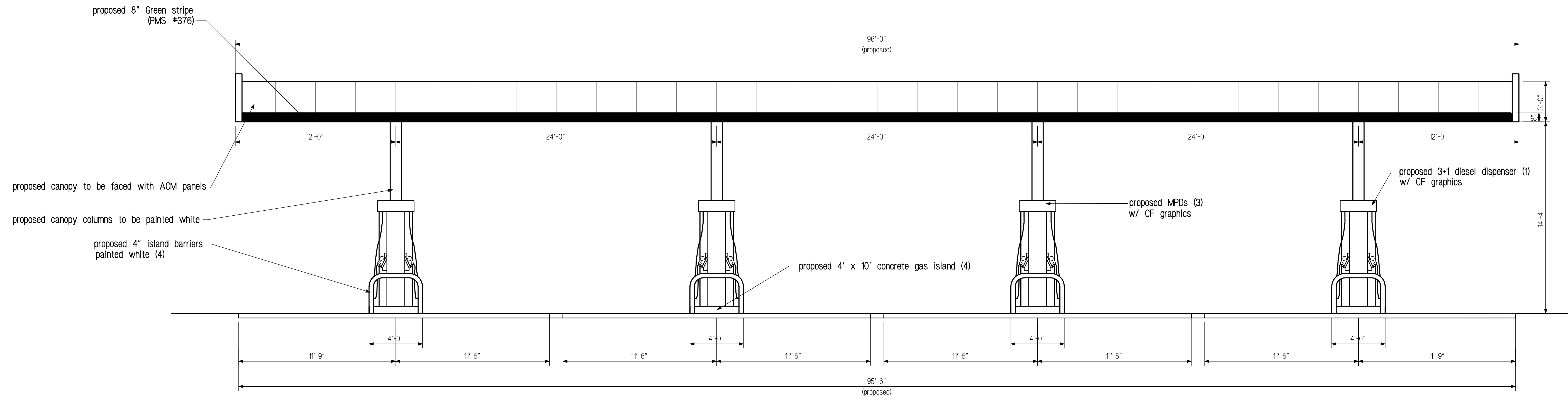
FRONT VIEW
