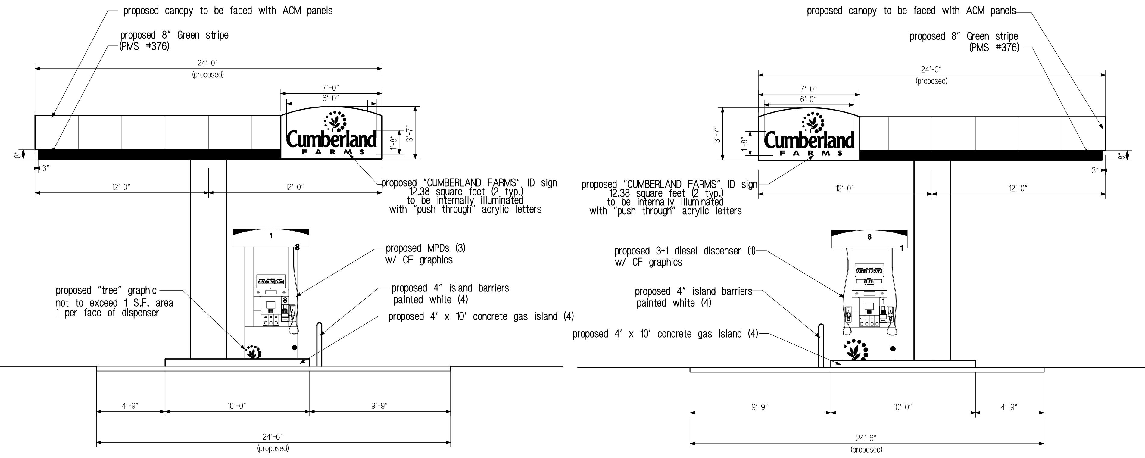
LEFT VIEW
