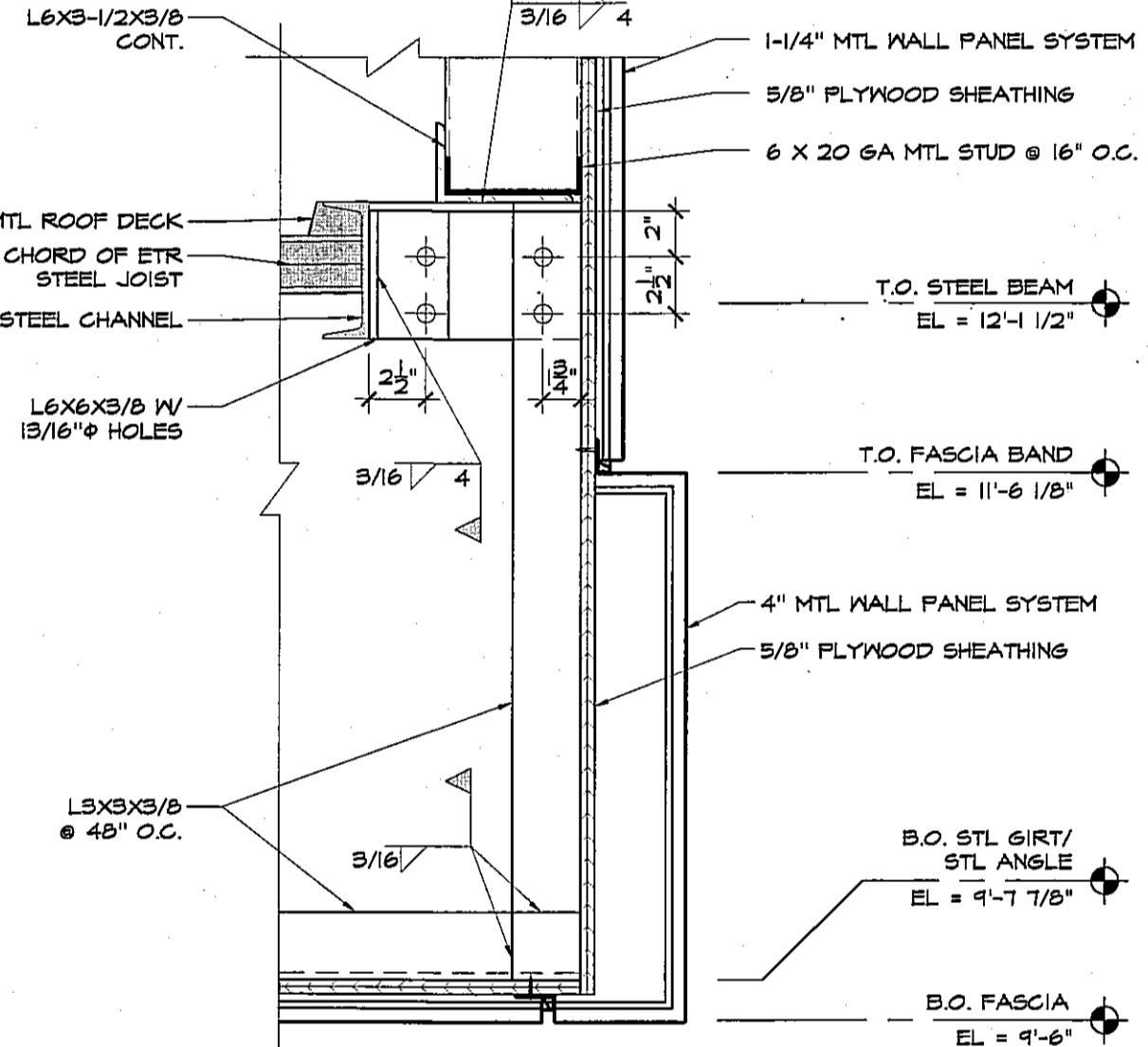
8 FASCIA DETAIL @ EXISTING A4.1 SCALE: 1/2" = 1'-0"
