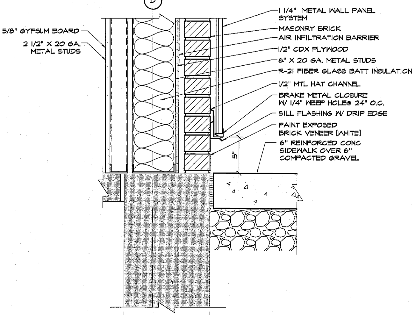
4 WALL BASE DETAIL A4.5 SCALE: 1/2" = 1'-0"
