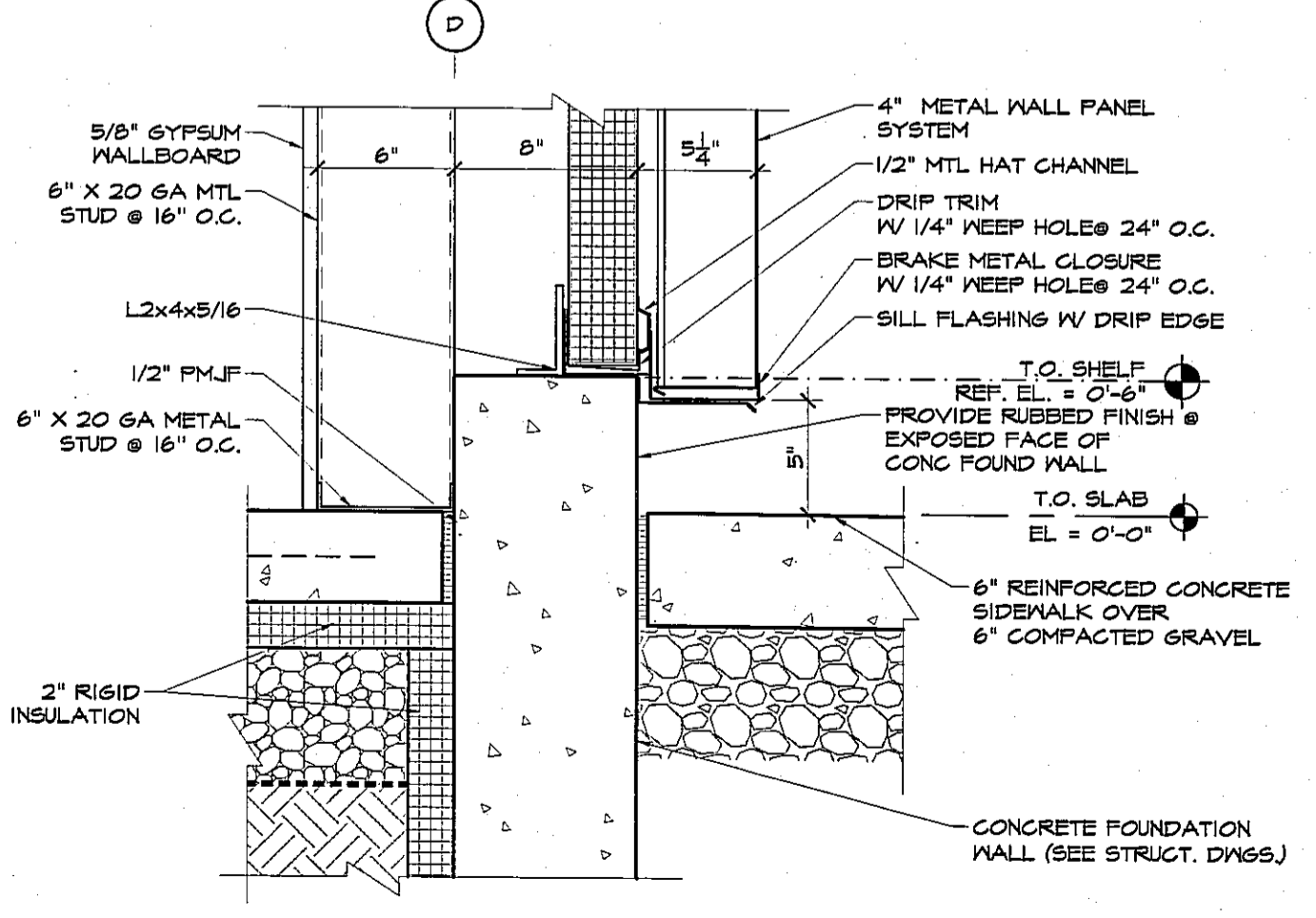
1 WALL BASE DETAIL A4.3 SCALE: 1/2" = 1'-0"
