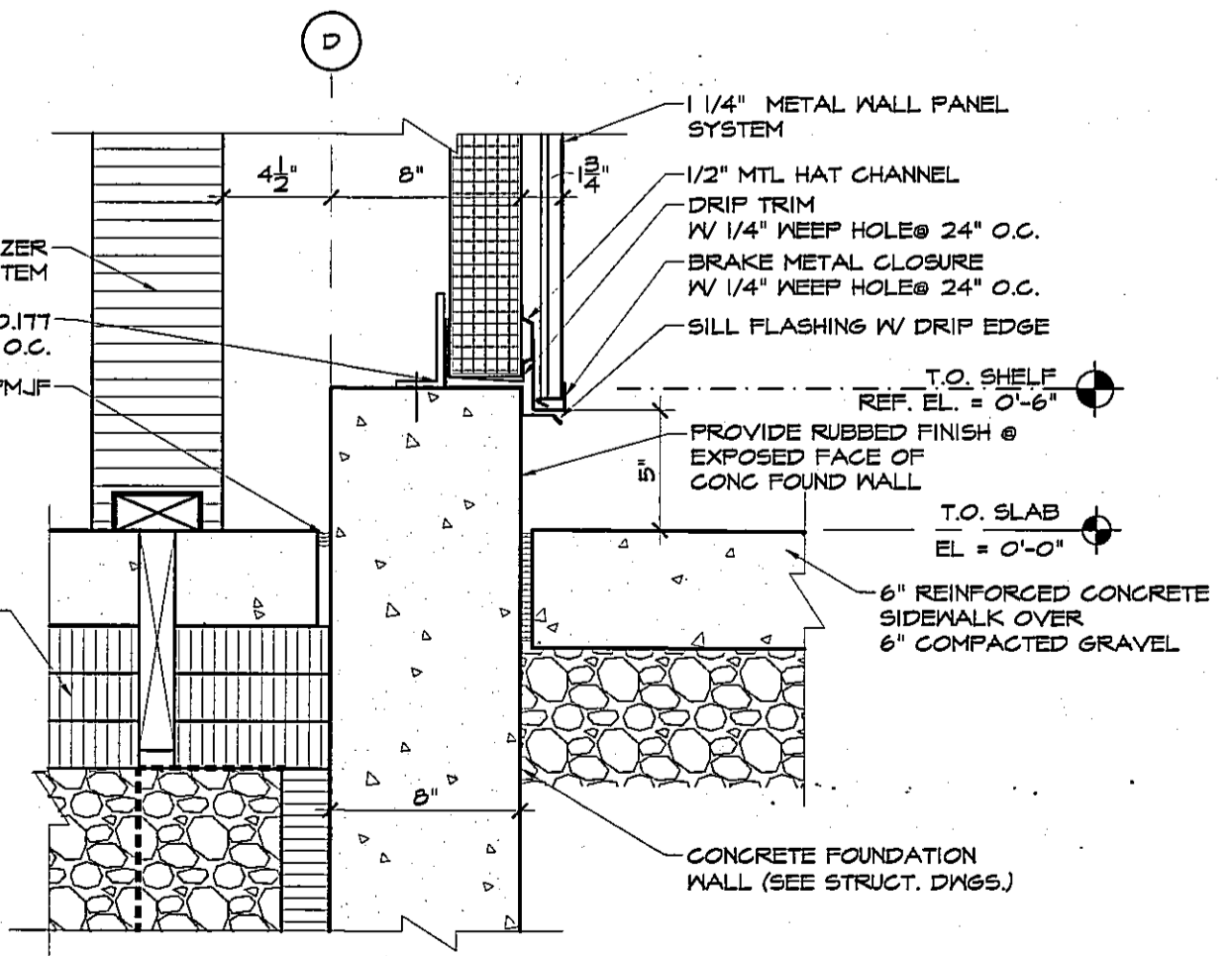
7 WALL BASE DETAIL A4.2 SCALE: 1/2" = 1'-0"
