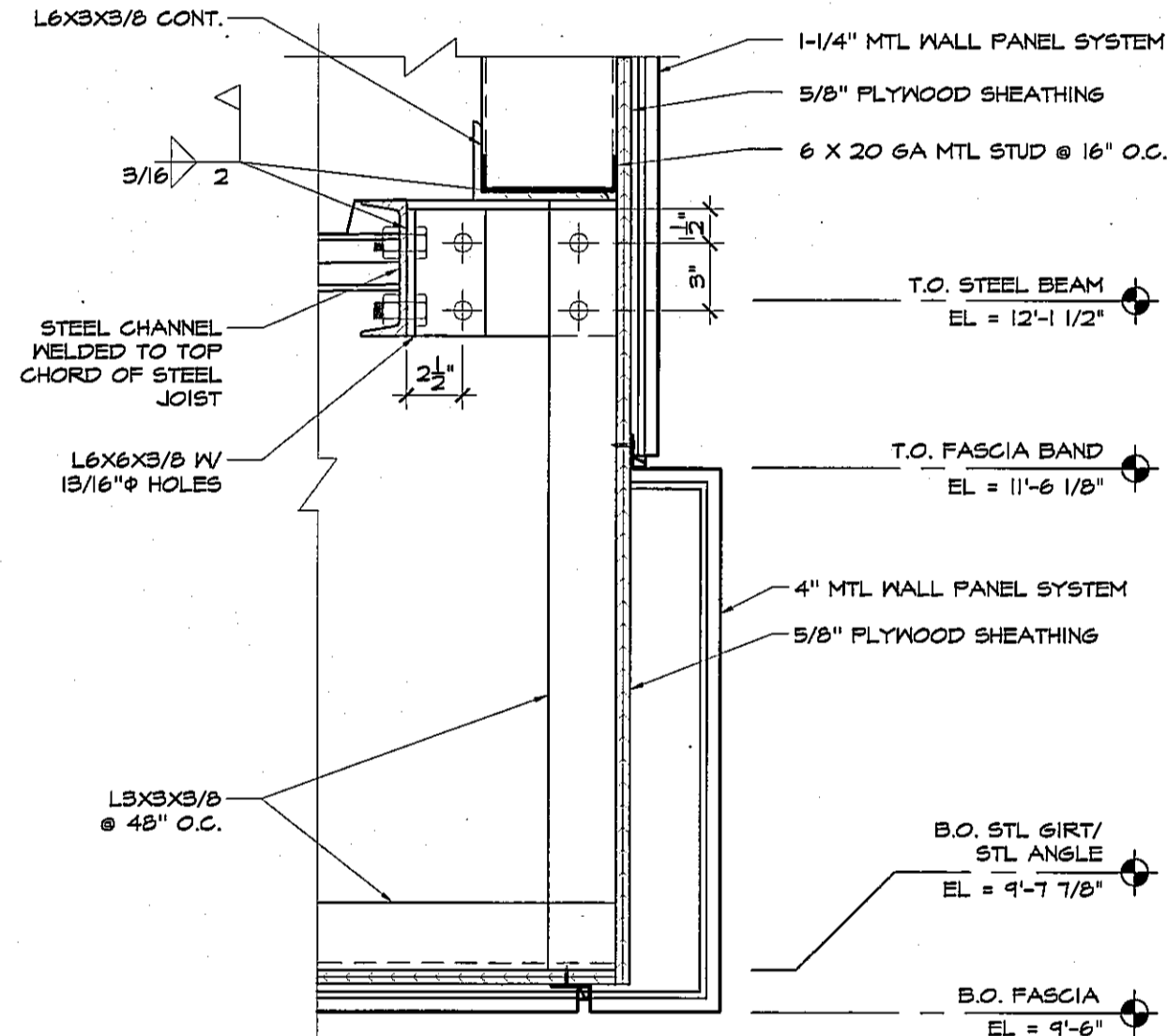
5 FASCIA DETAIL @ ADDITION A4.2 SCALE: 1/2" = 1'-0"
