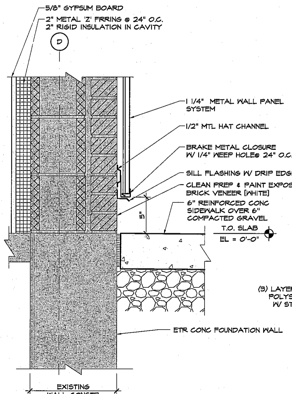
10 WALL BASE DETAIL A4.1 SCALE: 1/2" = 1'-0"
