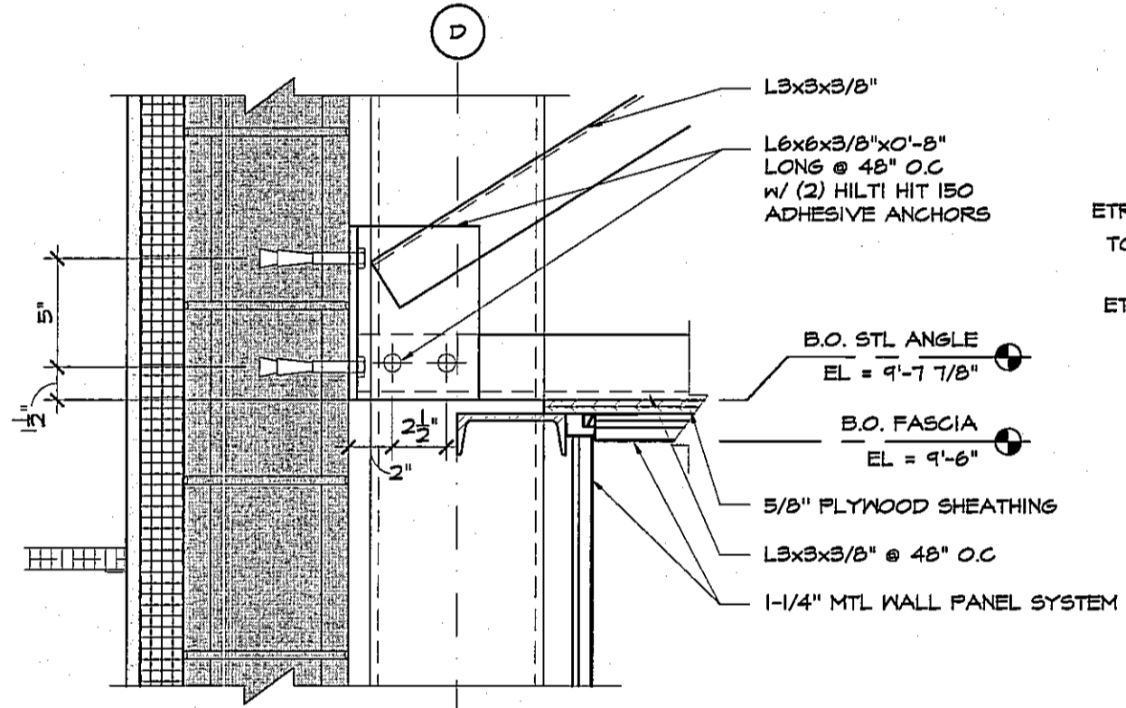
11 SOFFIT FRAMING DETAIL A4.1 SCALE: 1/2" = 1'-0"
