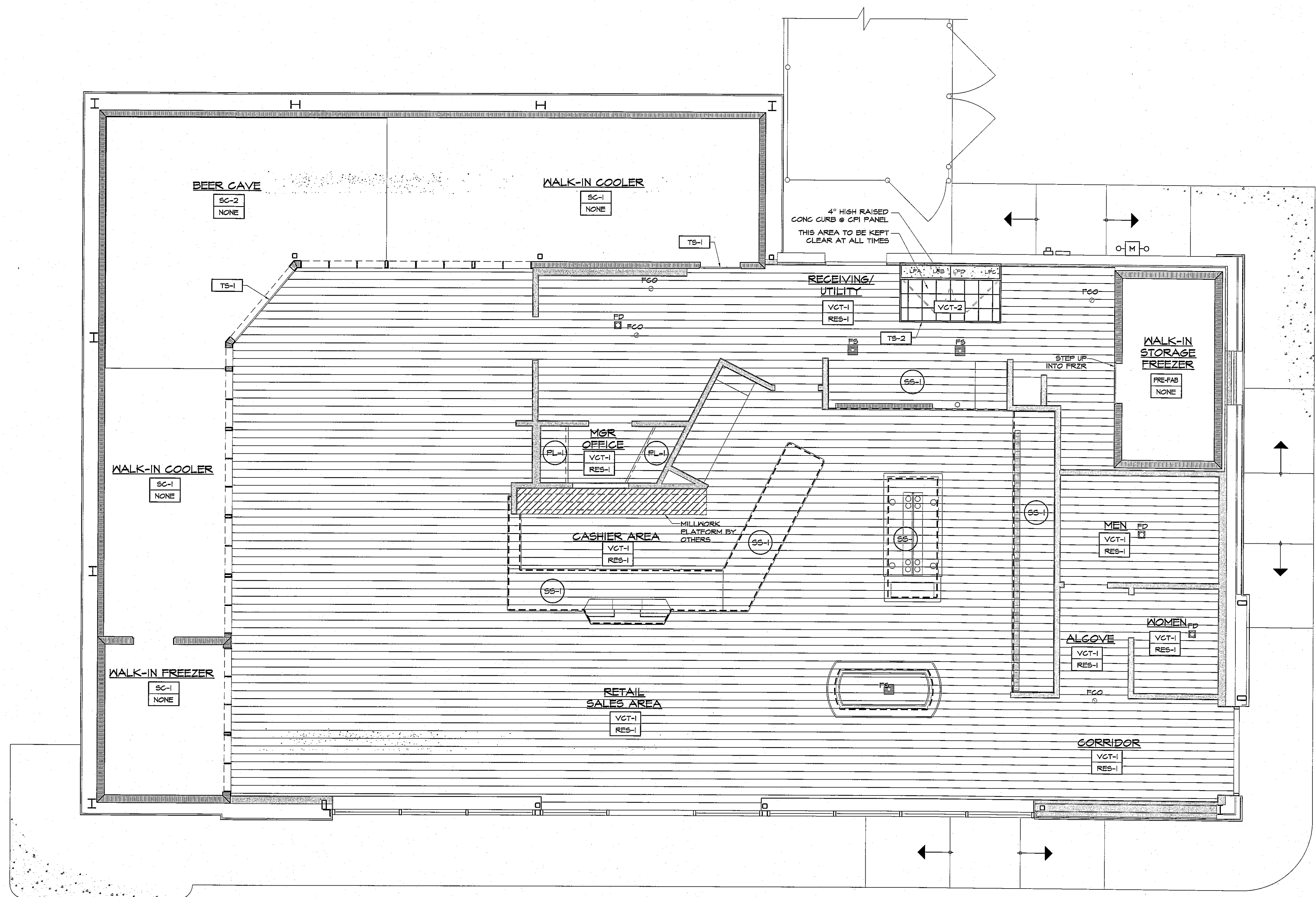
1 FLOOR FINISH PLAN SCALE: 1/4" = 1'-0" PLAN
