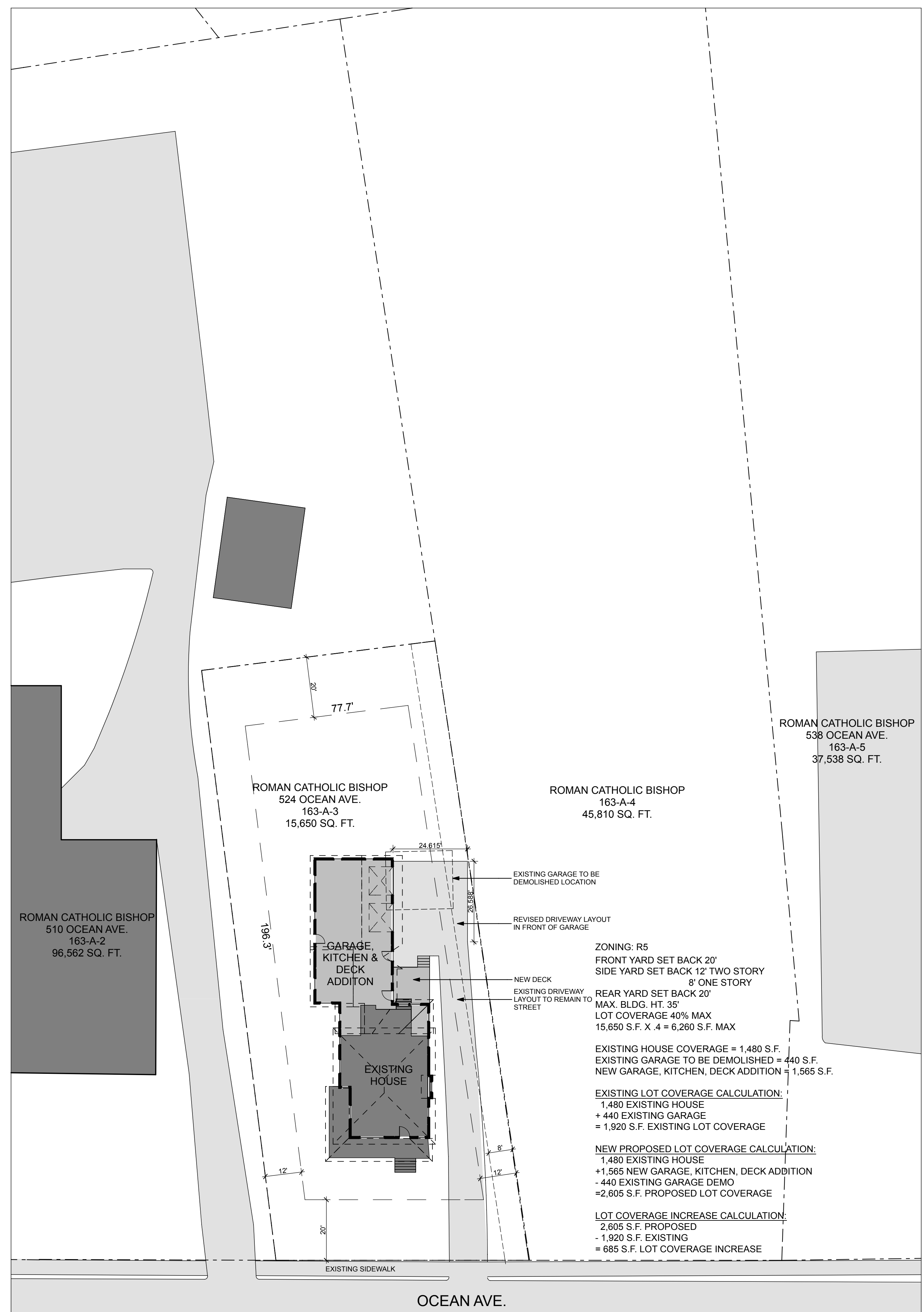
1 A1.1 PROPOSED SITE PLAN SCALE: 1" = 20'
