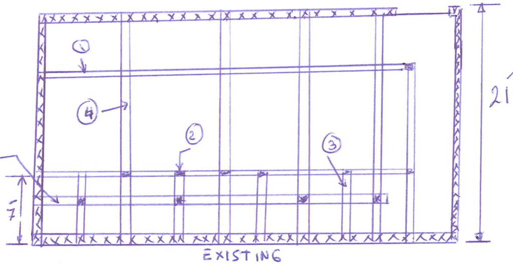
Top view of foundation
