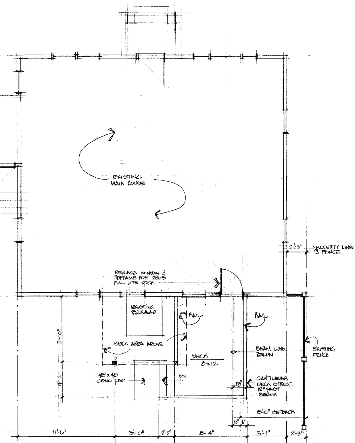
FIRST FLOOR/DECK PLAN 1/4"=1'-0"
