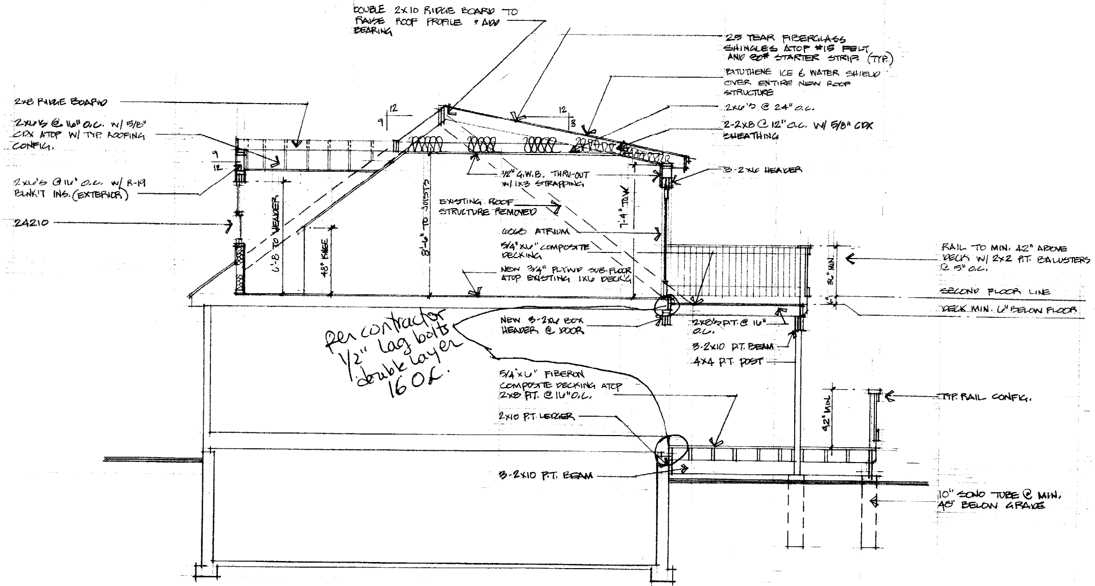
BUILDING SECTION 1/4" = 1'-0"
