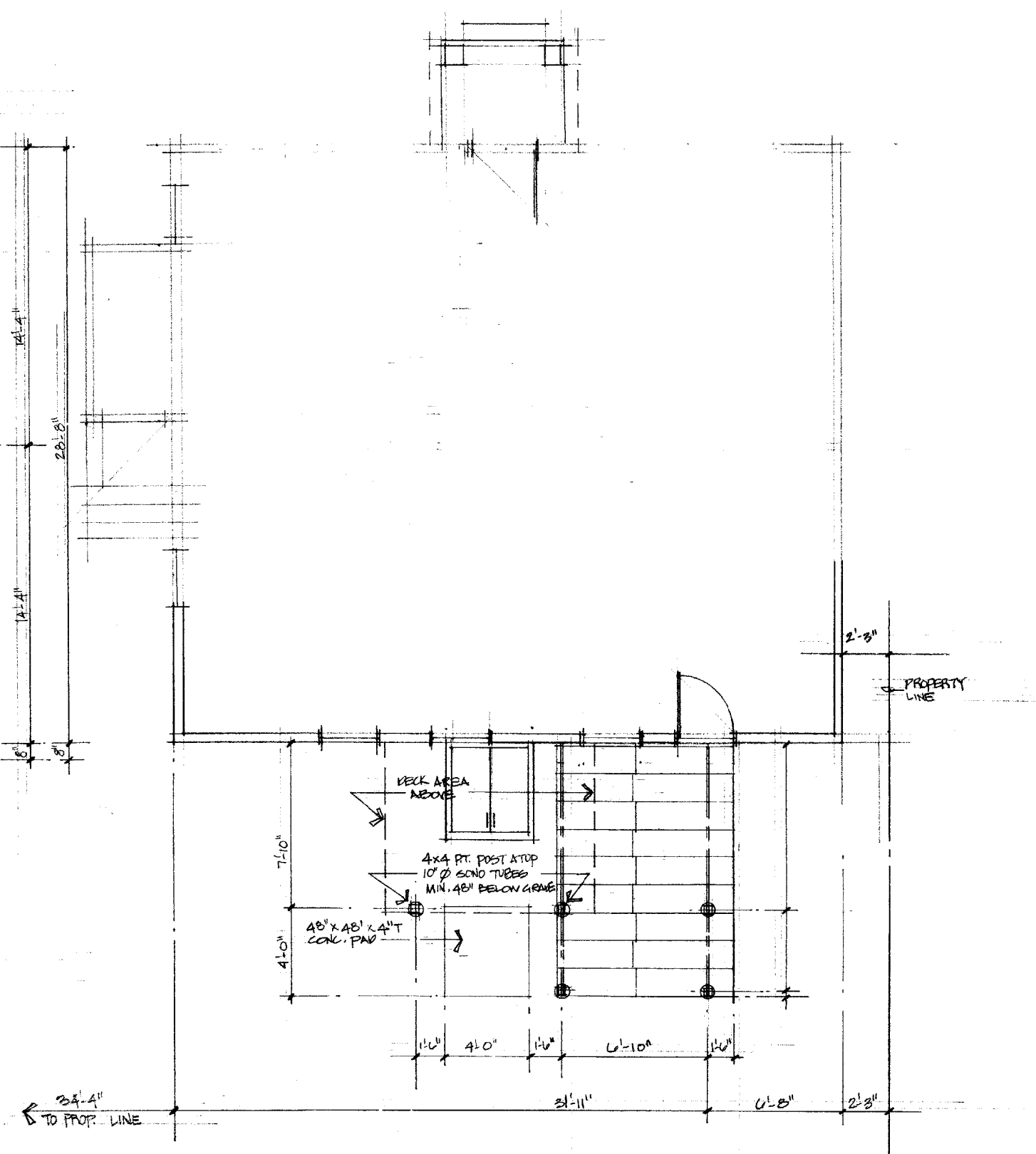
FOUNDATION / DECK FRAMING PLAN 1/4"=1'-0"
