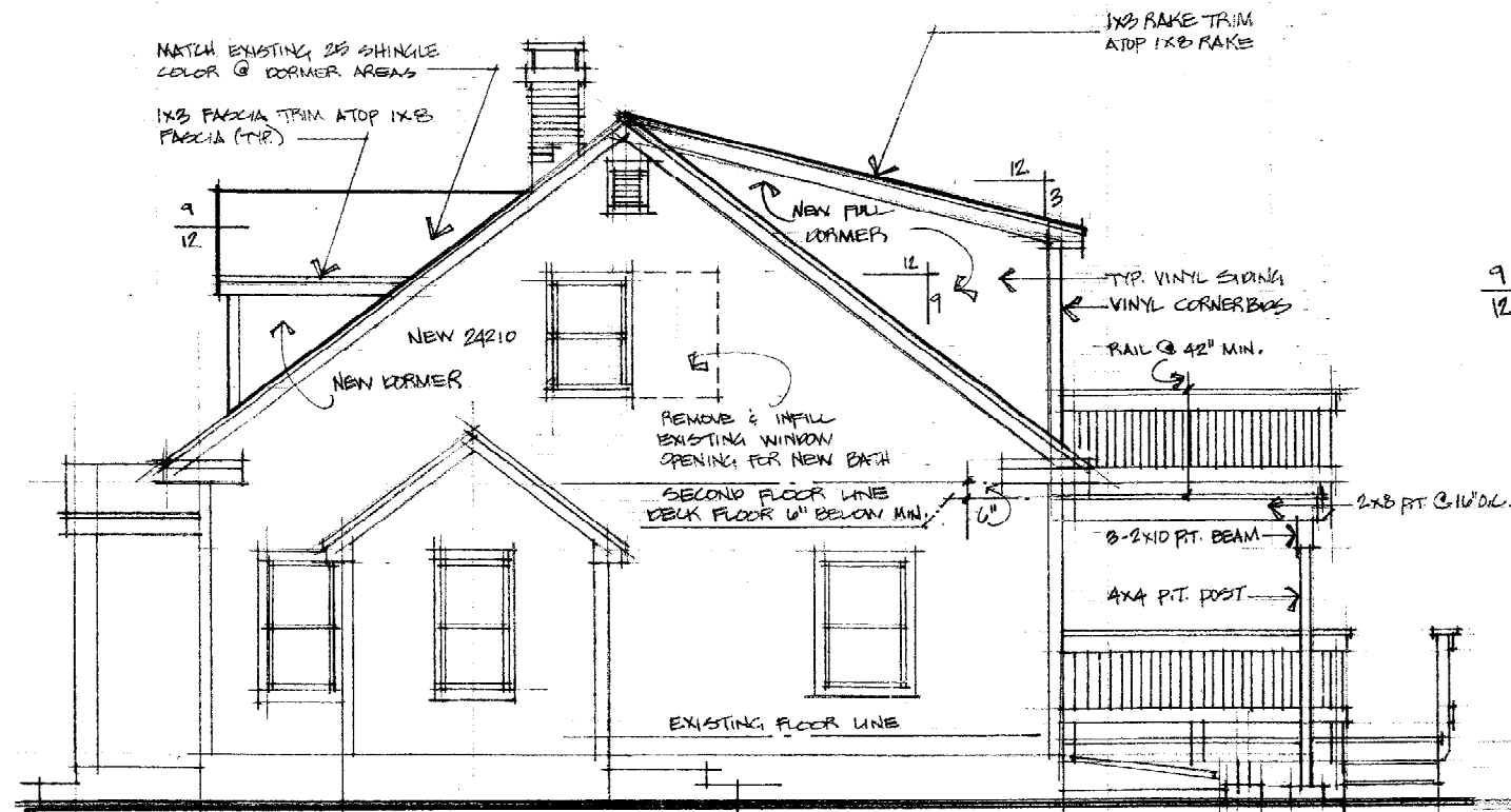
RIGHT ELEVATION 1/4" = 1'-0"
