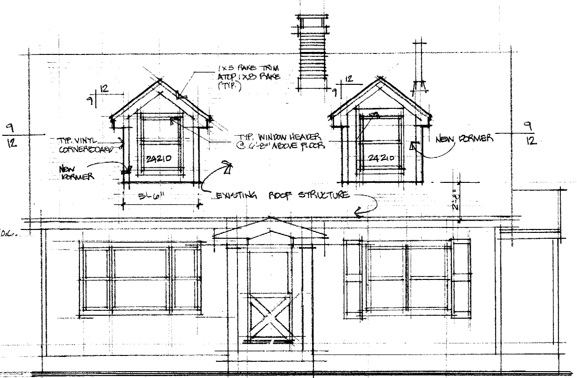
FRONT ELEVATION 1/4" = 1'-0"
