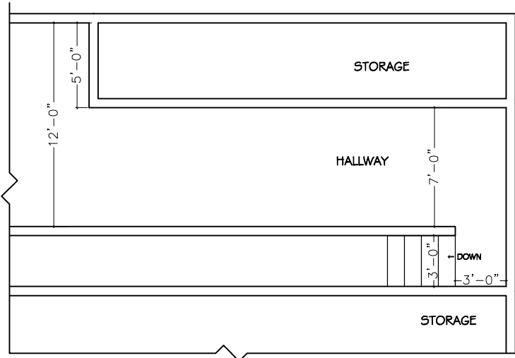
EXISTING FLOOR PLAN SCALE: 1/8" = 1'-0"
