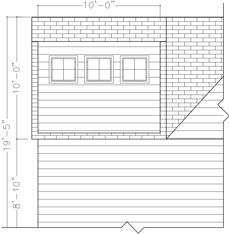
PROPOSED ELEVATIONS SCALE: 1/4" = 1'-0"
