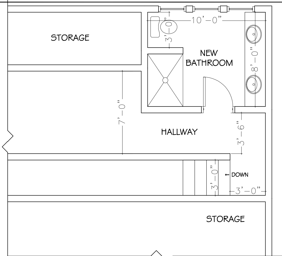
PROPOSED BATHROOM FLOOR PLAN SCALE: 1/4" = 1'-0"
