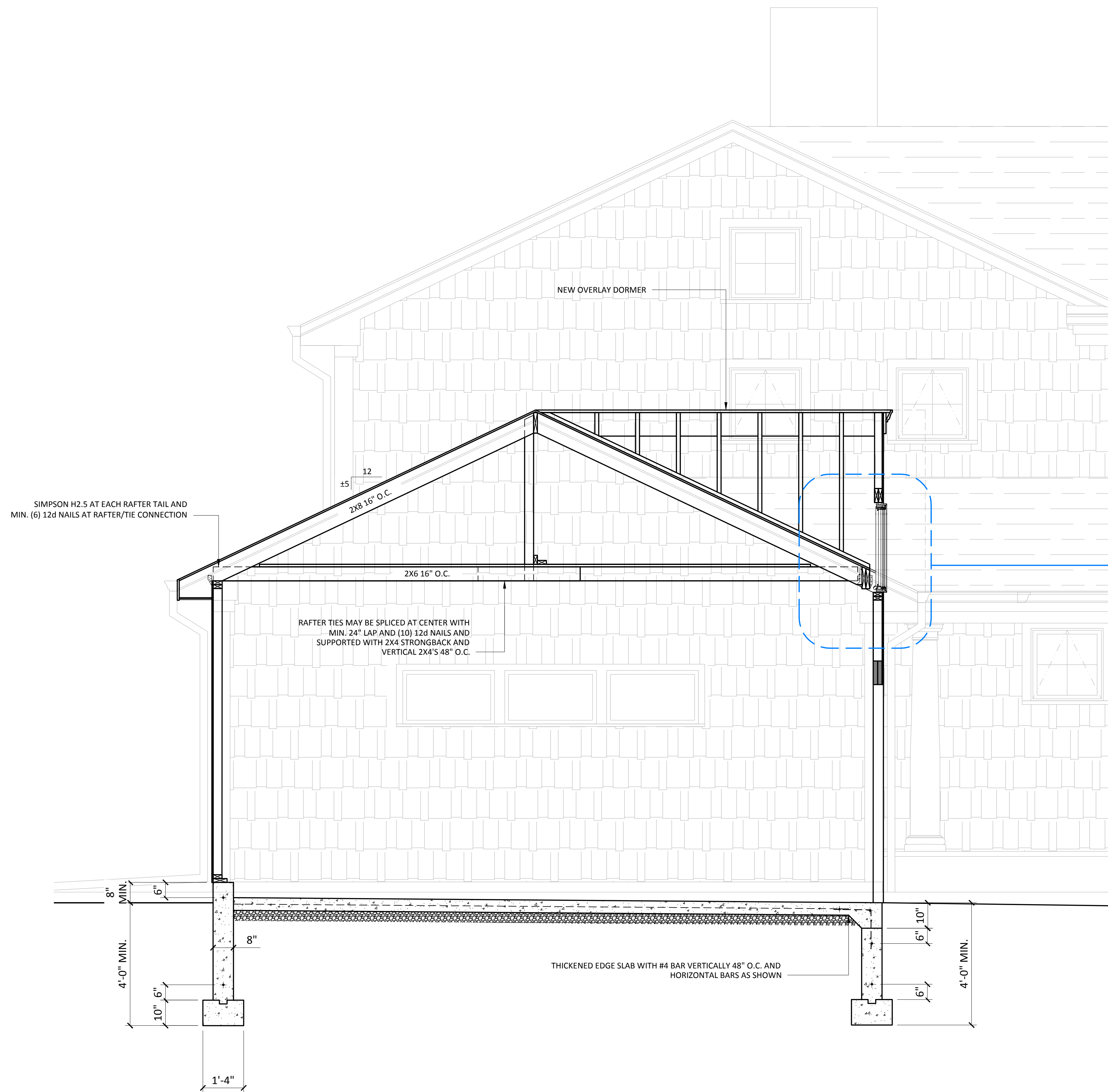
1 SECTION 3-3 1/2" = 1'-0"
