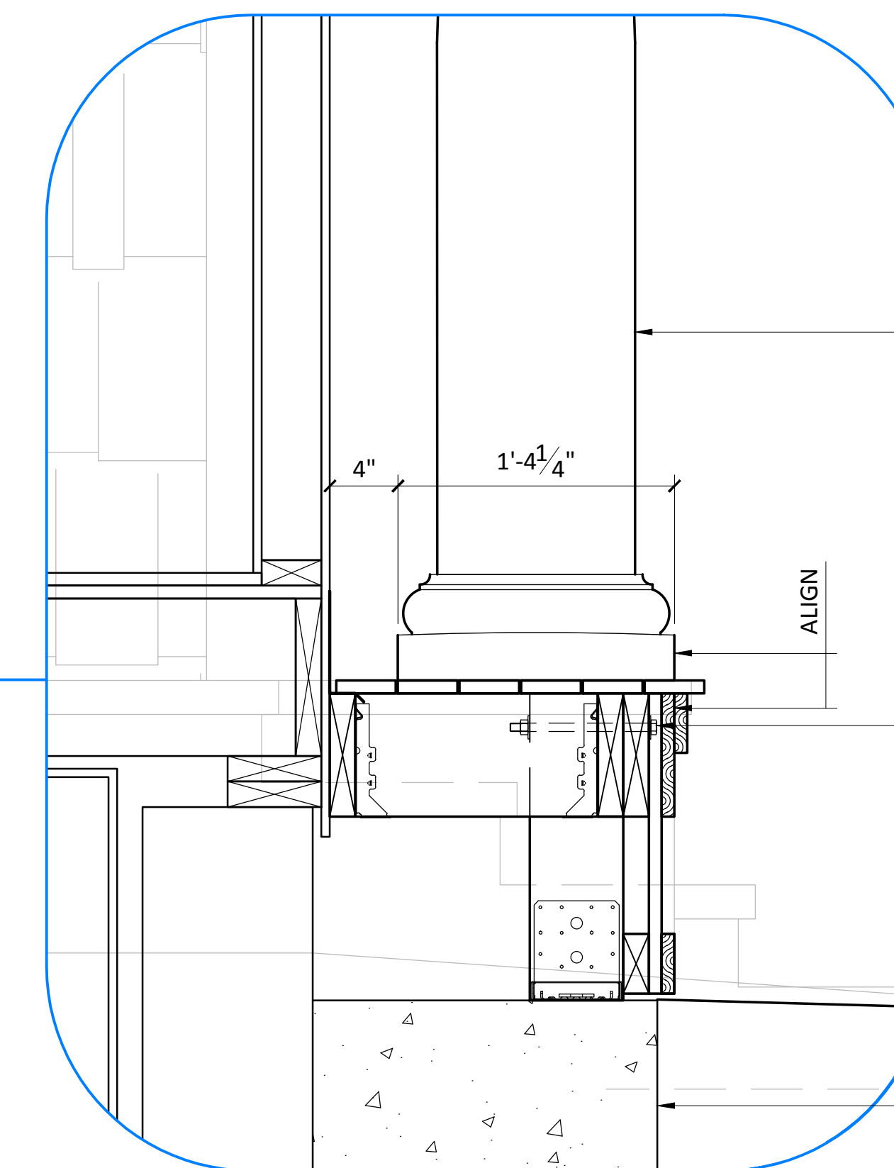
2 DETAILS 1 1/2" = 1'-0"
