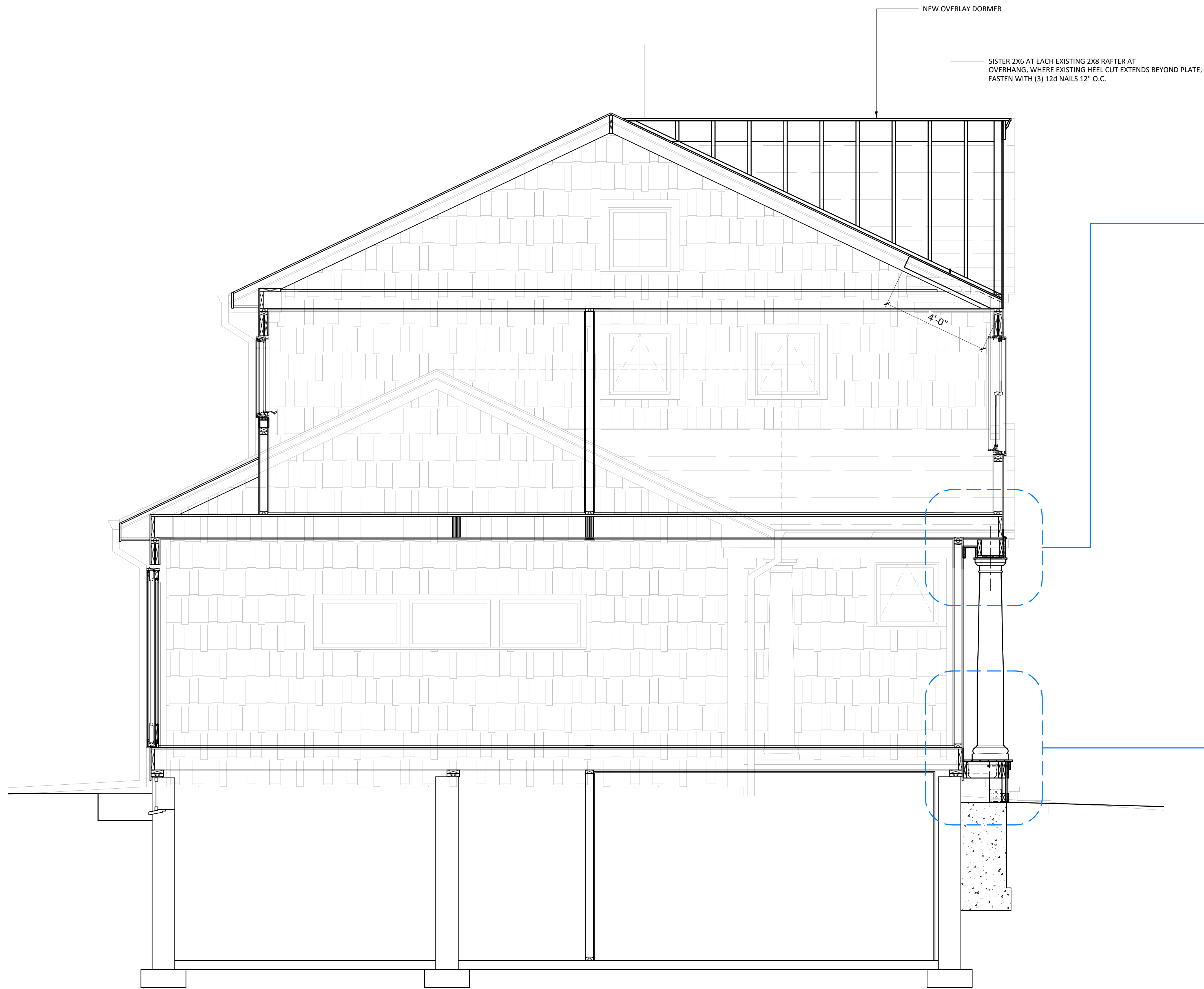
1 SECTION 2-2 1/2" = 1'-0"
