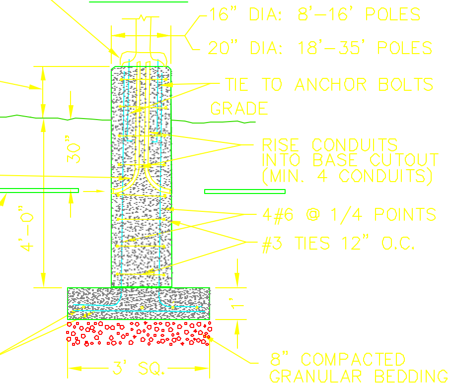
PRECAST CONCRETE LIGHT POLE BASE
