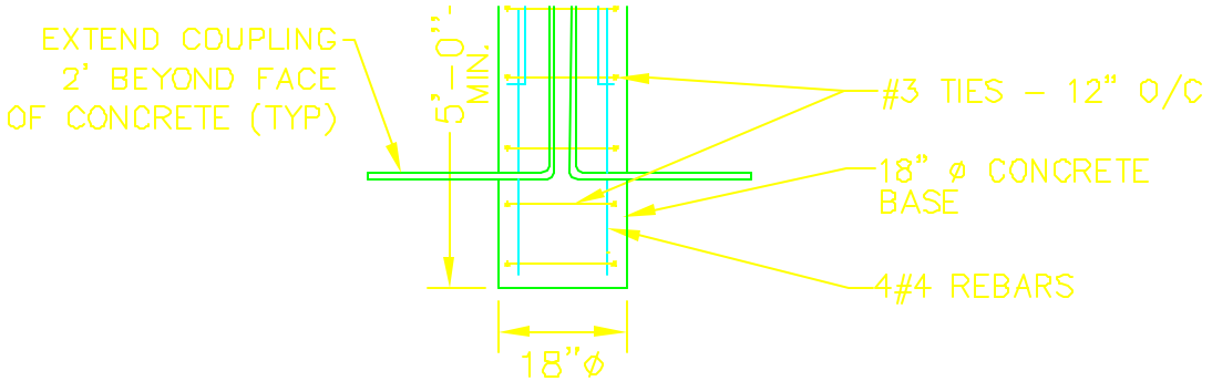
LIGHT BOLLARD/FIXTURE DETAIL
