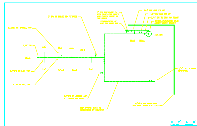
PLUMBING SUPPLY PLAN CONCESSION STAND SCALE 1/4" = 1'-0"
