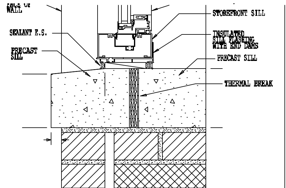
SILL DETAIL
