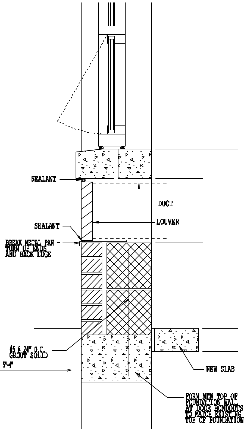
SILL DETAIL
