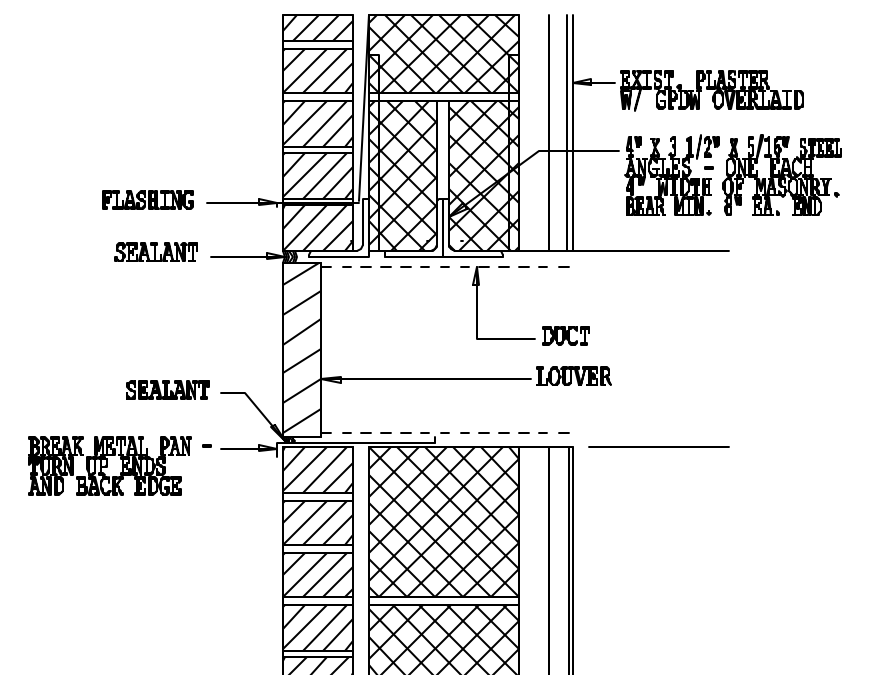
UNIT VENTILATOR LOUVER DETAIL
