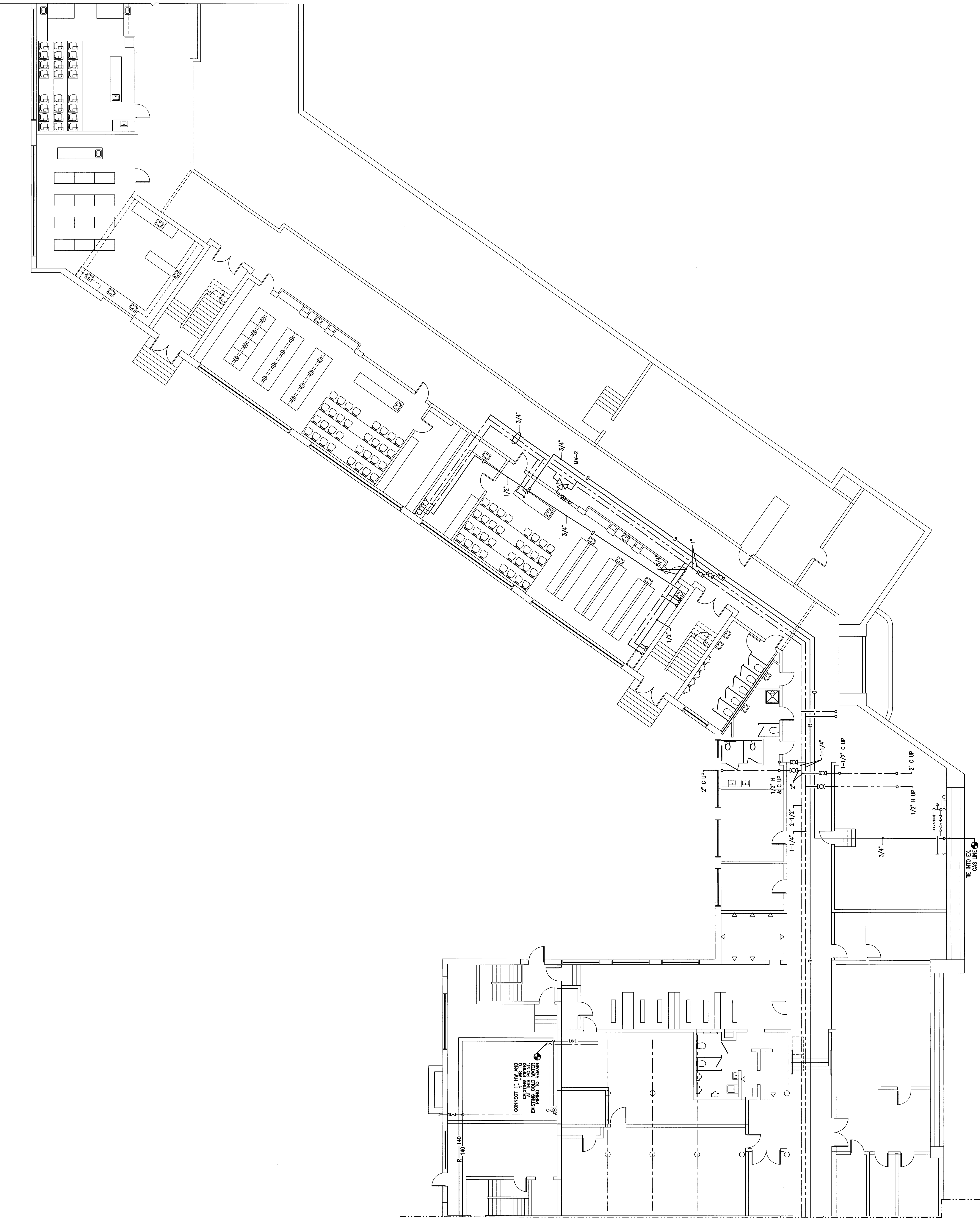
GROUND FLOOR AREA "B" H & C PIPING PLAN SCALE: 1/8" = 1'-0"
