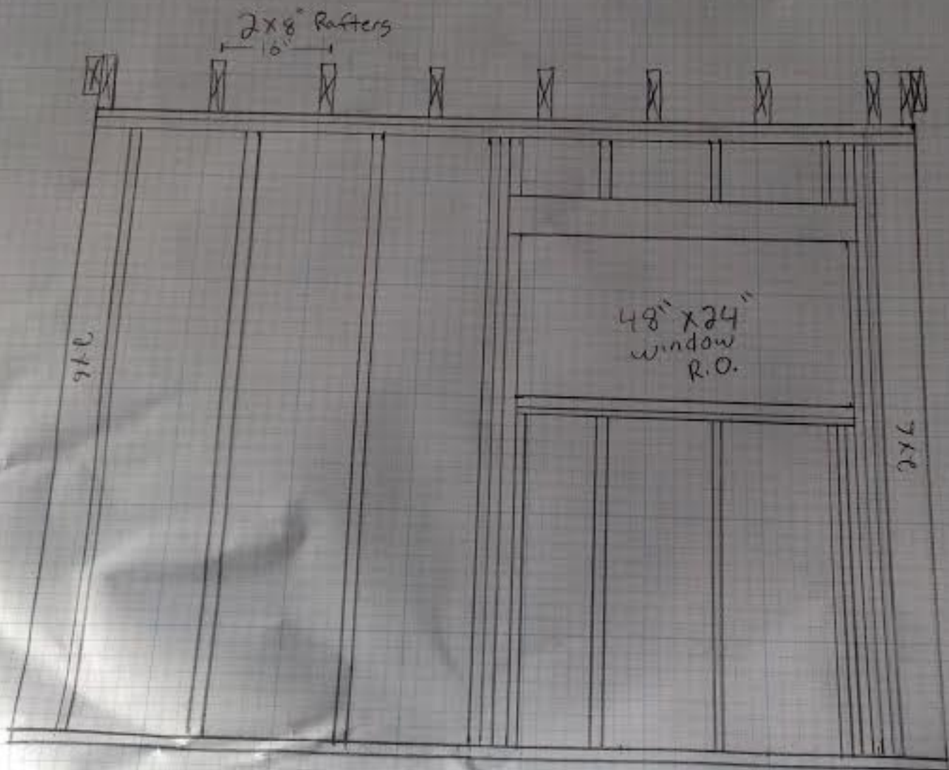
Back Wall Elevation framing
