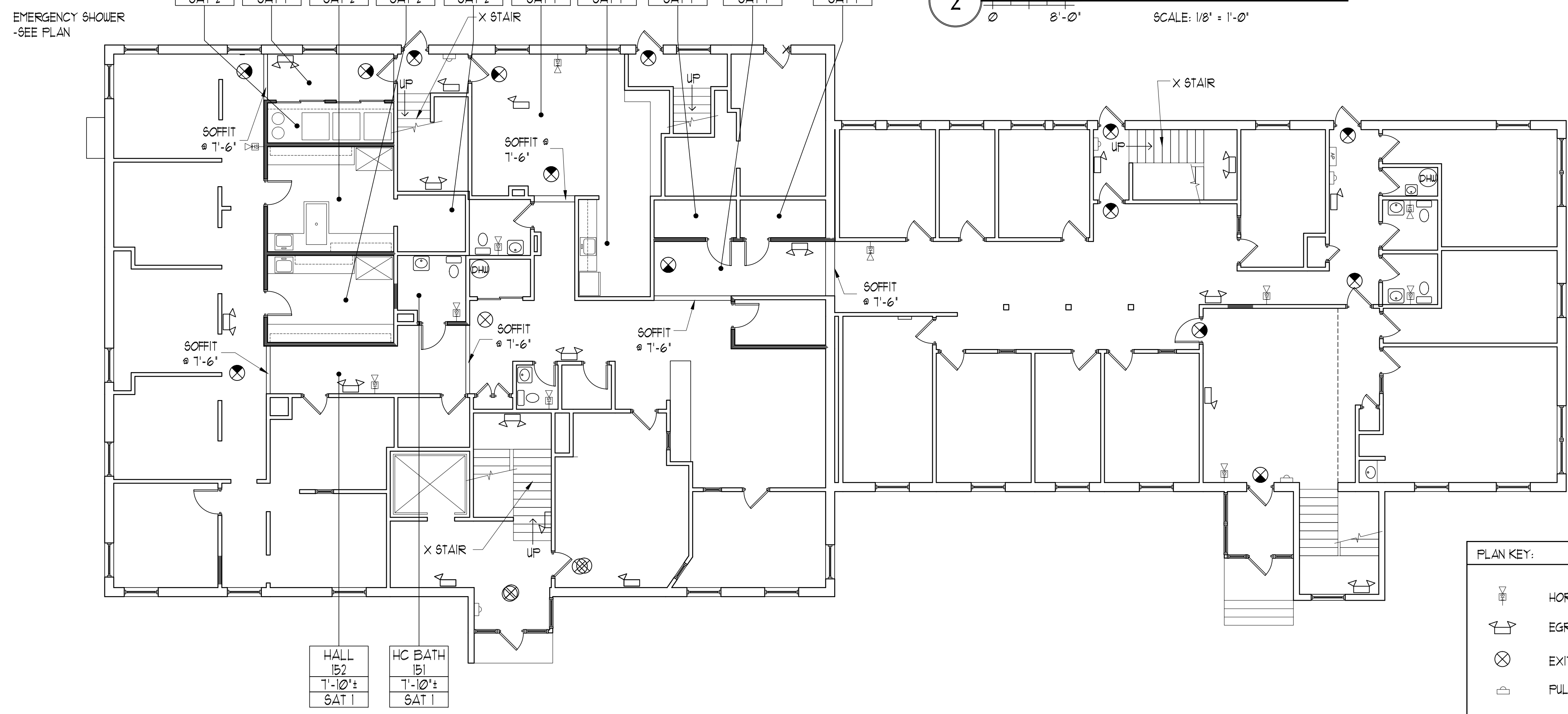
1 FIRST FLOOR - RCP SCALE: 1/8" = 1'-0"
