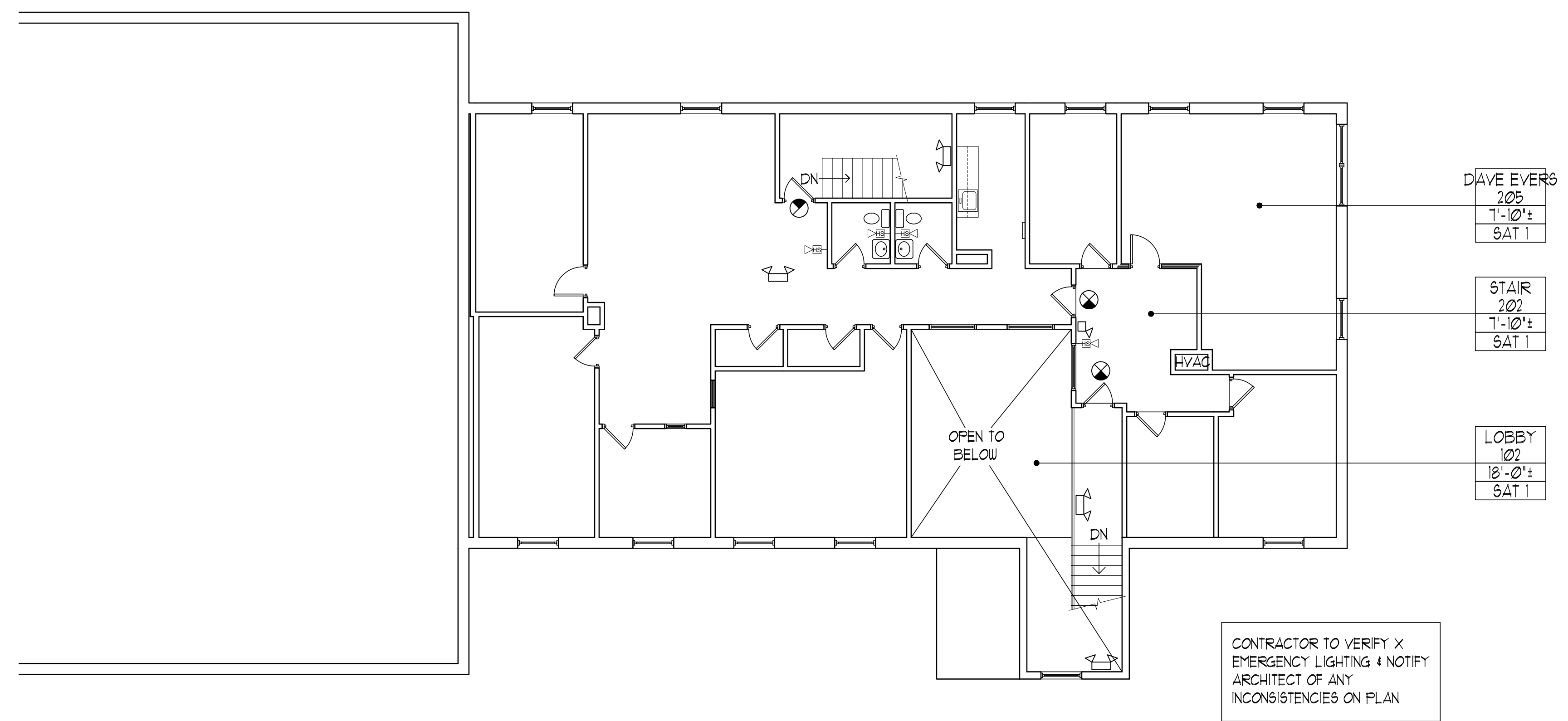
2 SECOND FLOOR - RCP SCALE: 1/8" = 1'-0"
