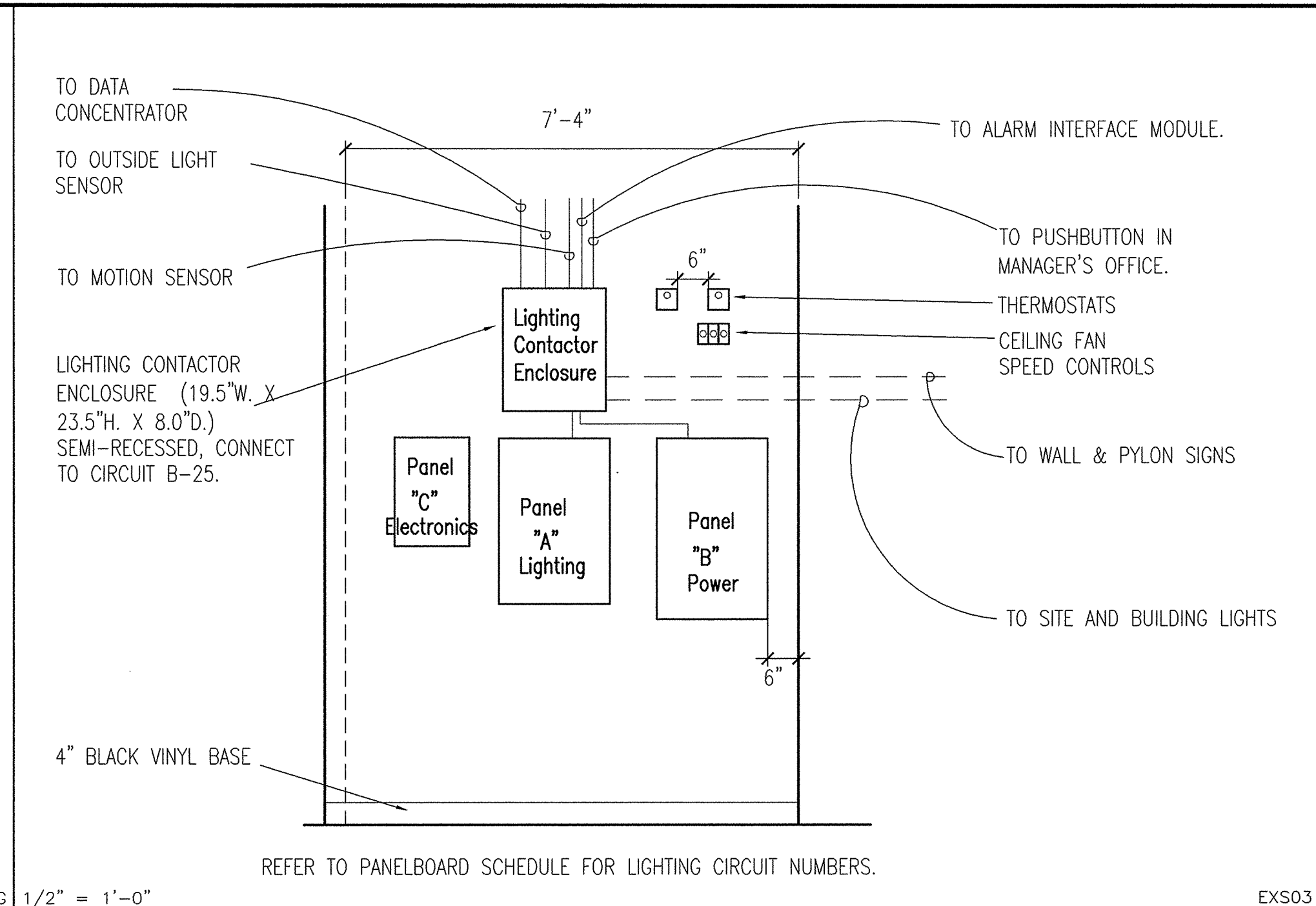
2 | PANELBOARD - DIAGRAM
