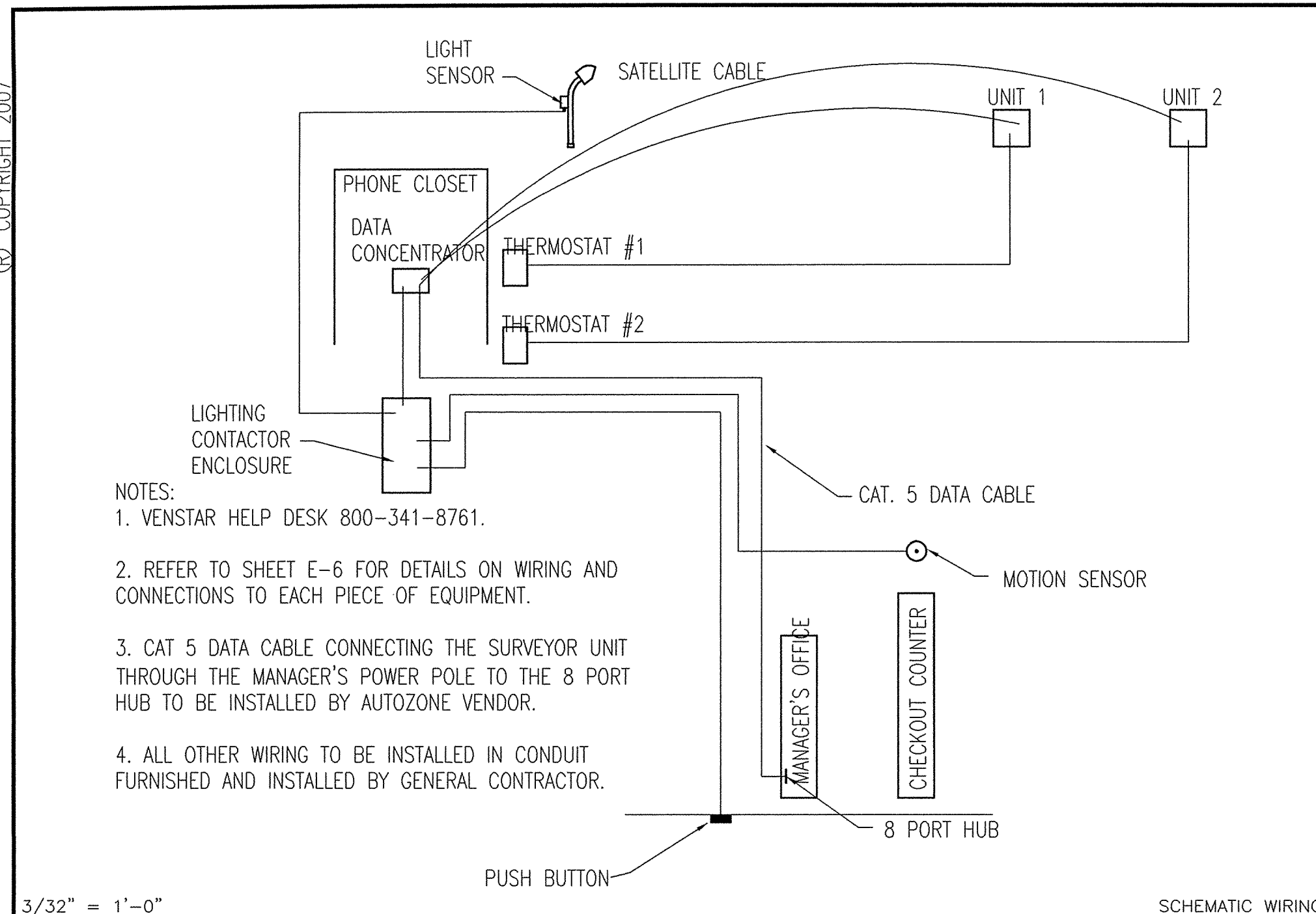
1 | SCHEMATIC WIRING DIAGRAM - VENSTAR / LIGHTING CONTROL PANEL
