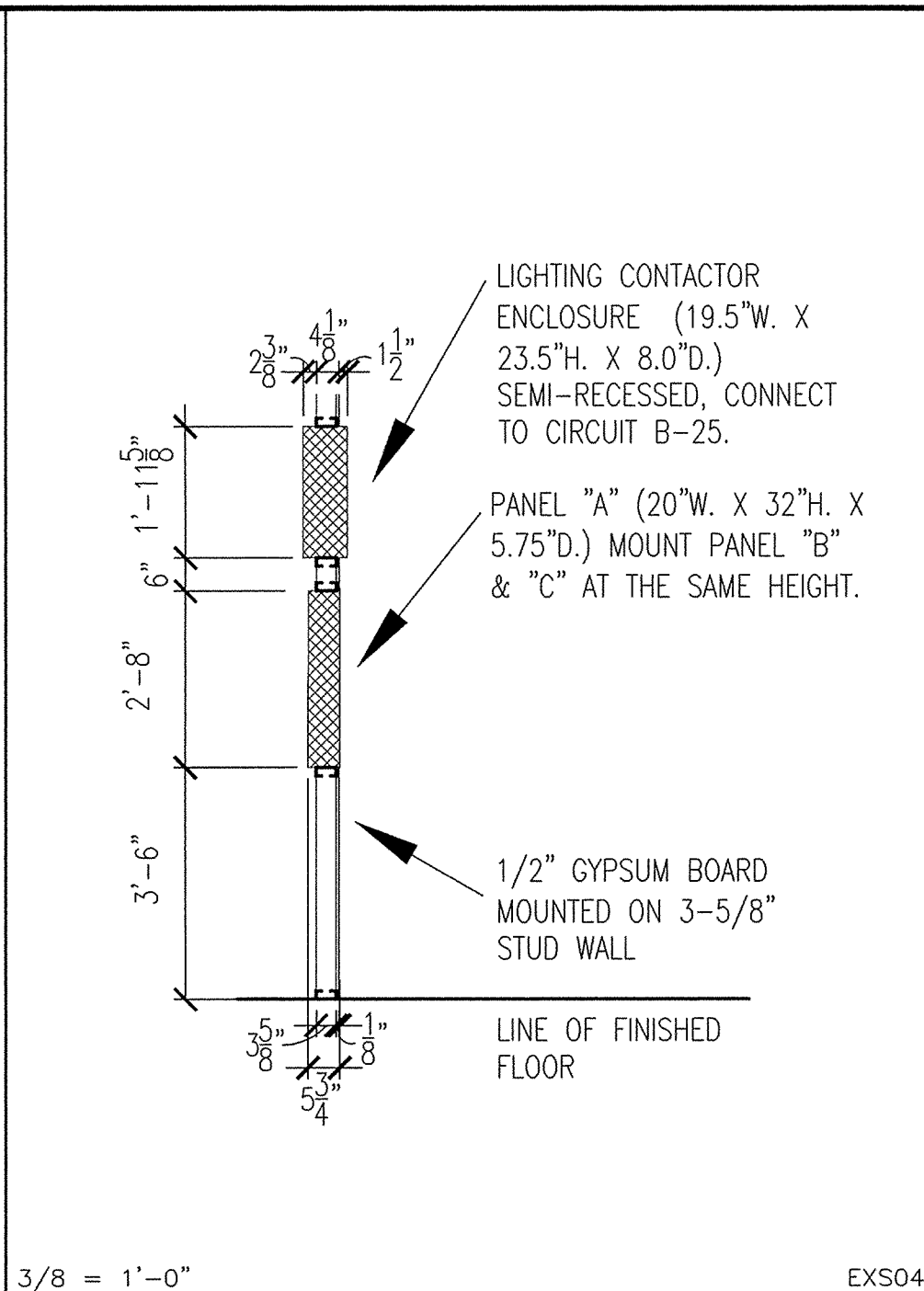
3 | PANELBOARD - MOUNTING HEIGHT SECTION
