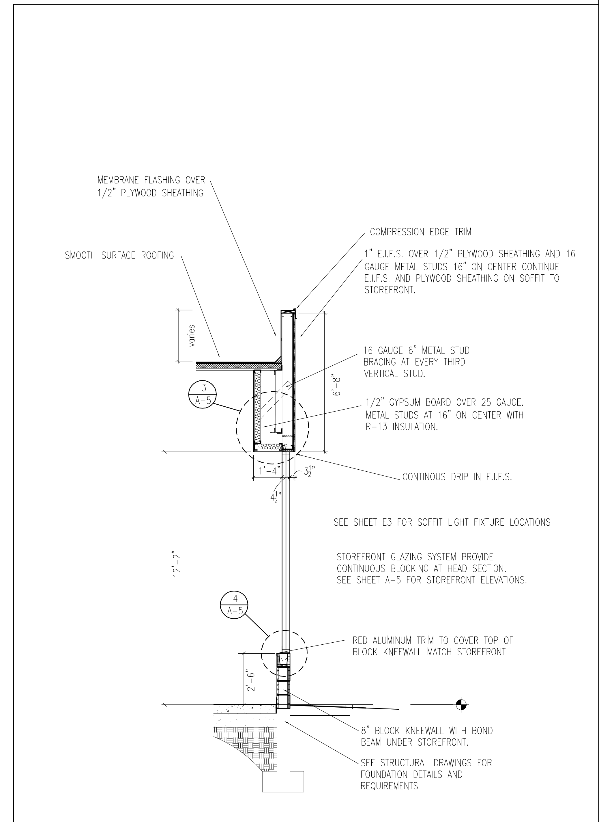
3/8" = 1'-0" 1 WALL SECTION - SIDE WALL (storefront) AWS04N
