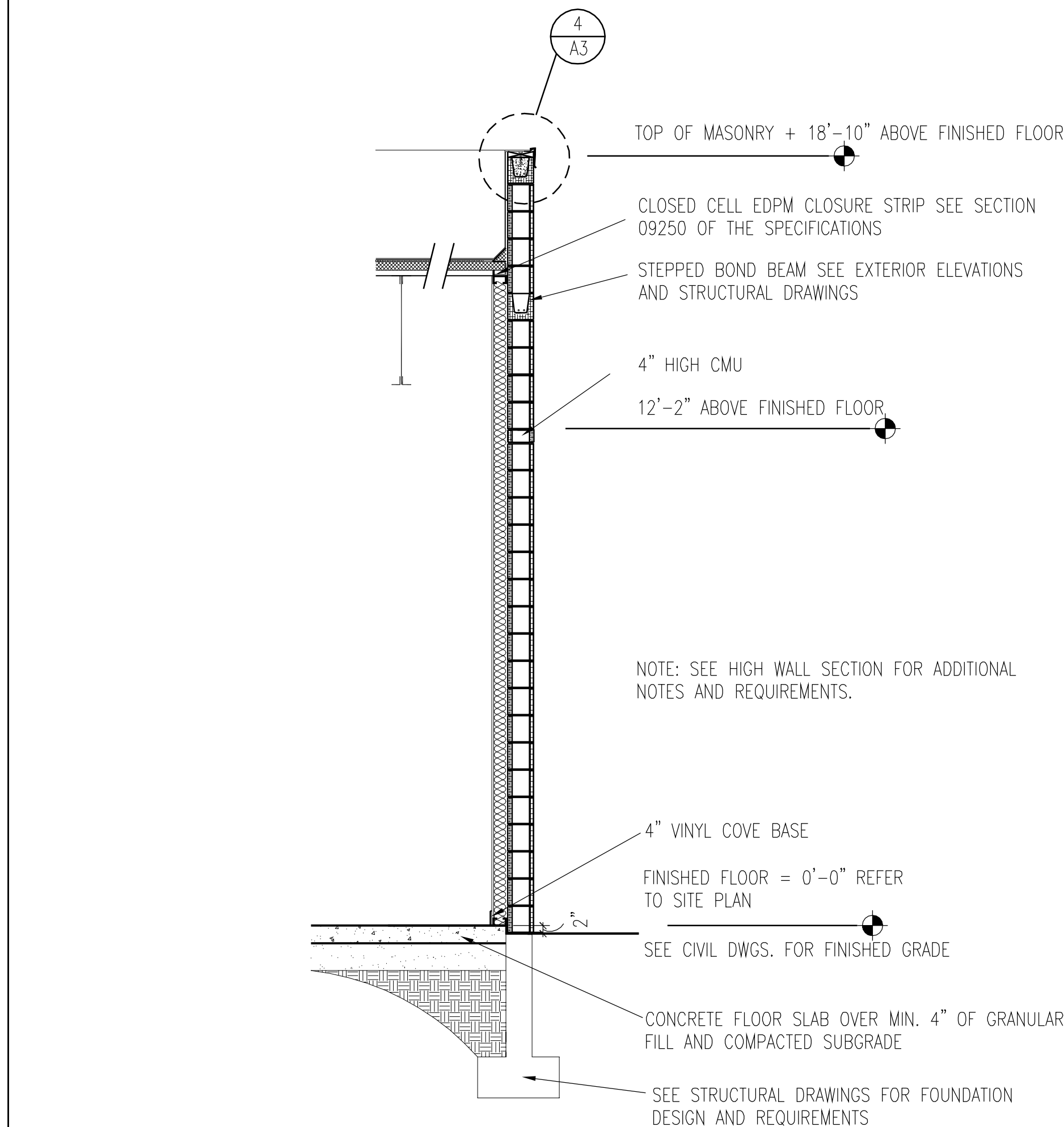
3/8" = 1'-0" 2 WALL SECTION END WALL
