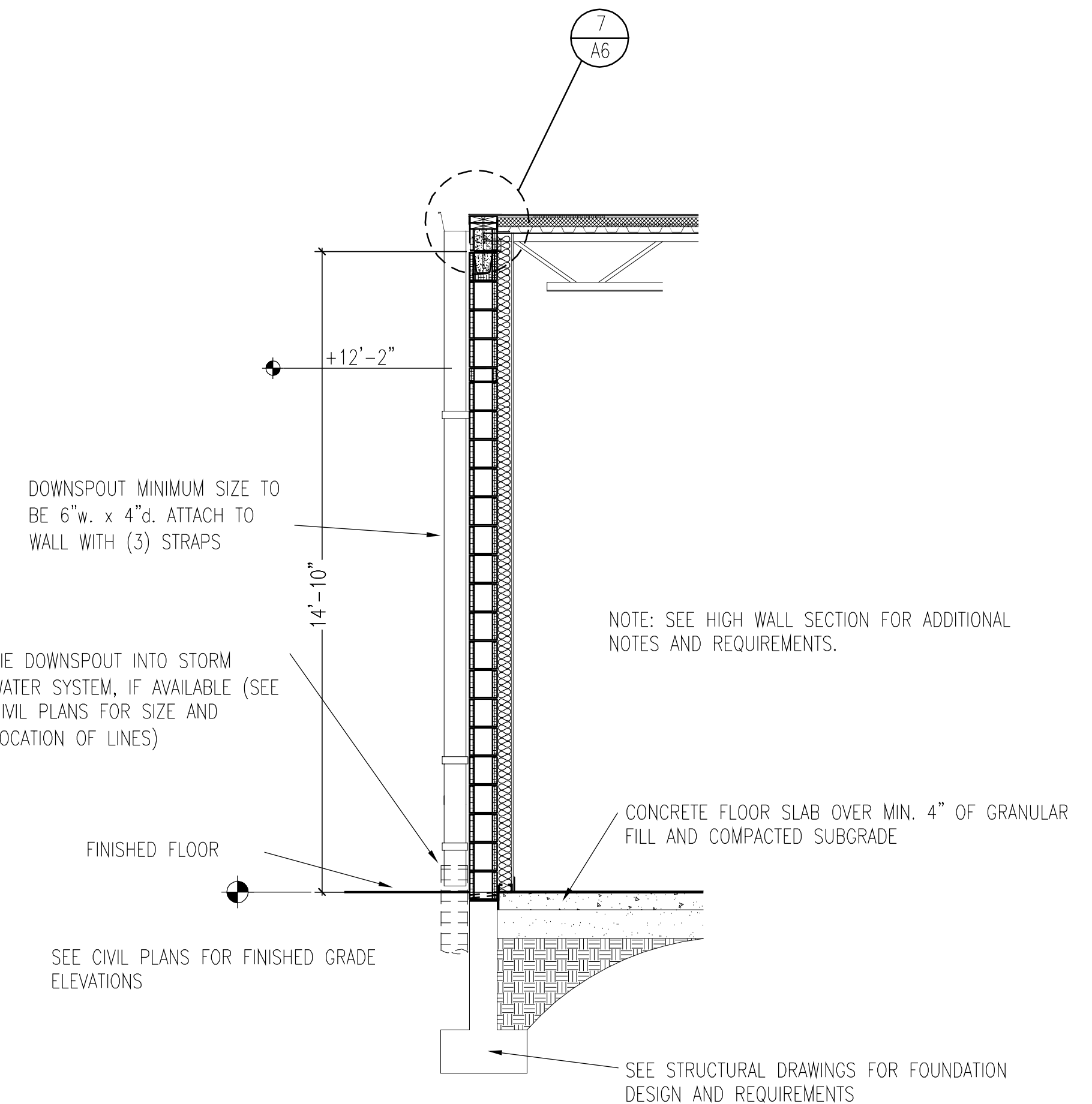
3/8" = 1'-0" 3 WALL SECTION LOW SIDE
