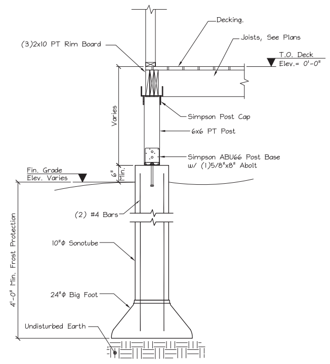
SECTION 3 EXTERIOR POST BASE (PIER) Scale: 3/4" = 1'-0"
