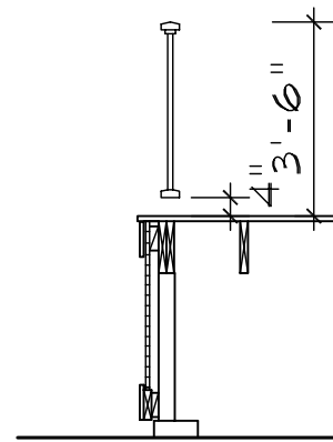
TYP. GUARDRAIL
