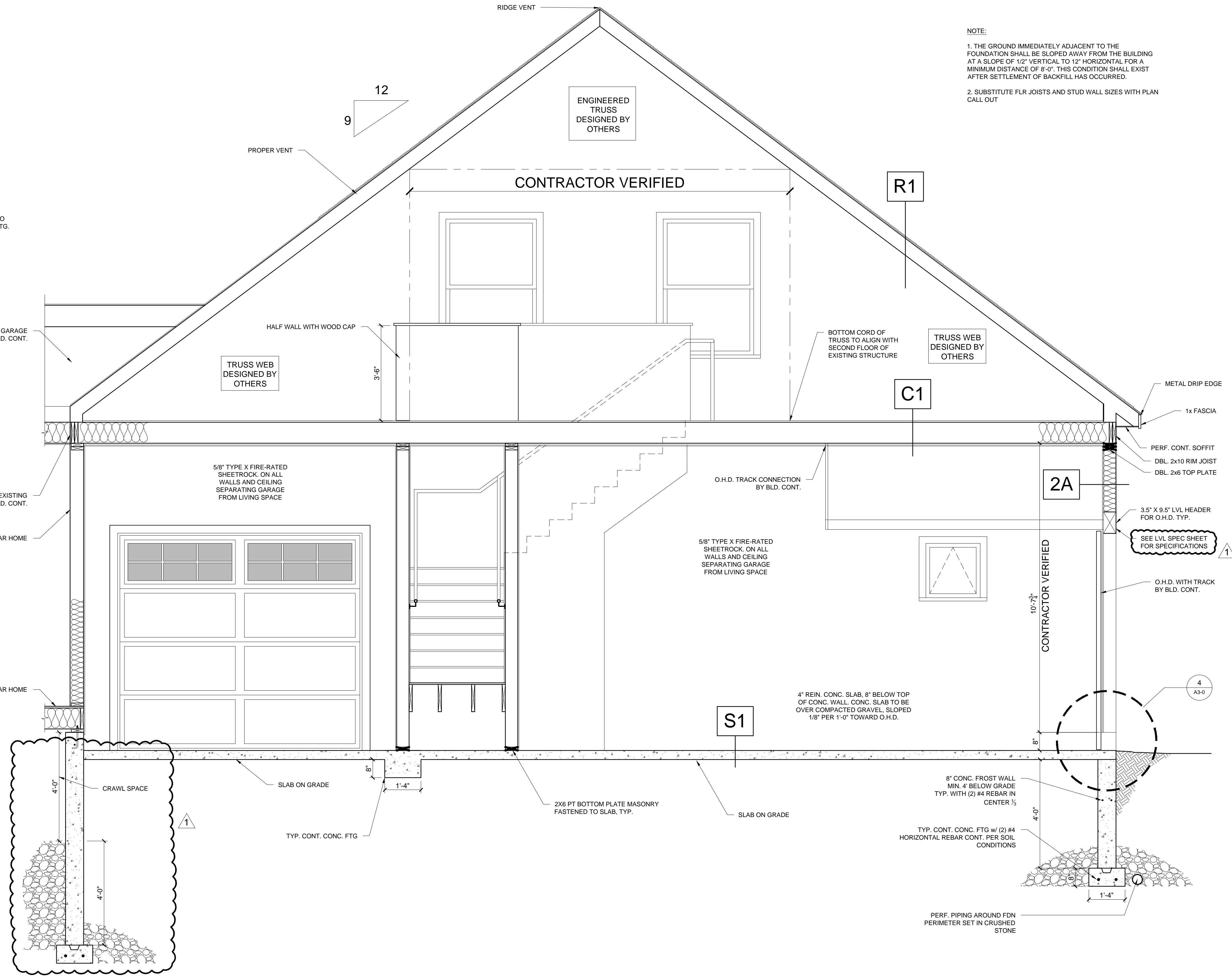
1 GARAGE SECTION 1/2" = 1'-0"
