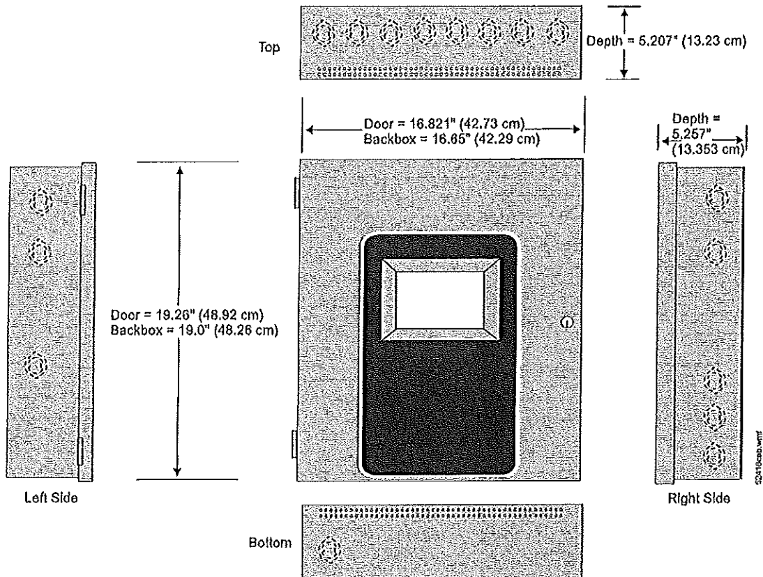
Cabinet Measurements
