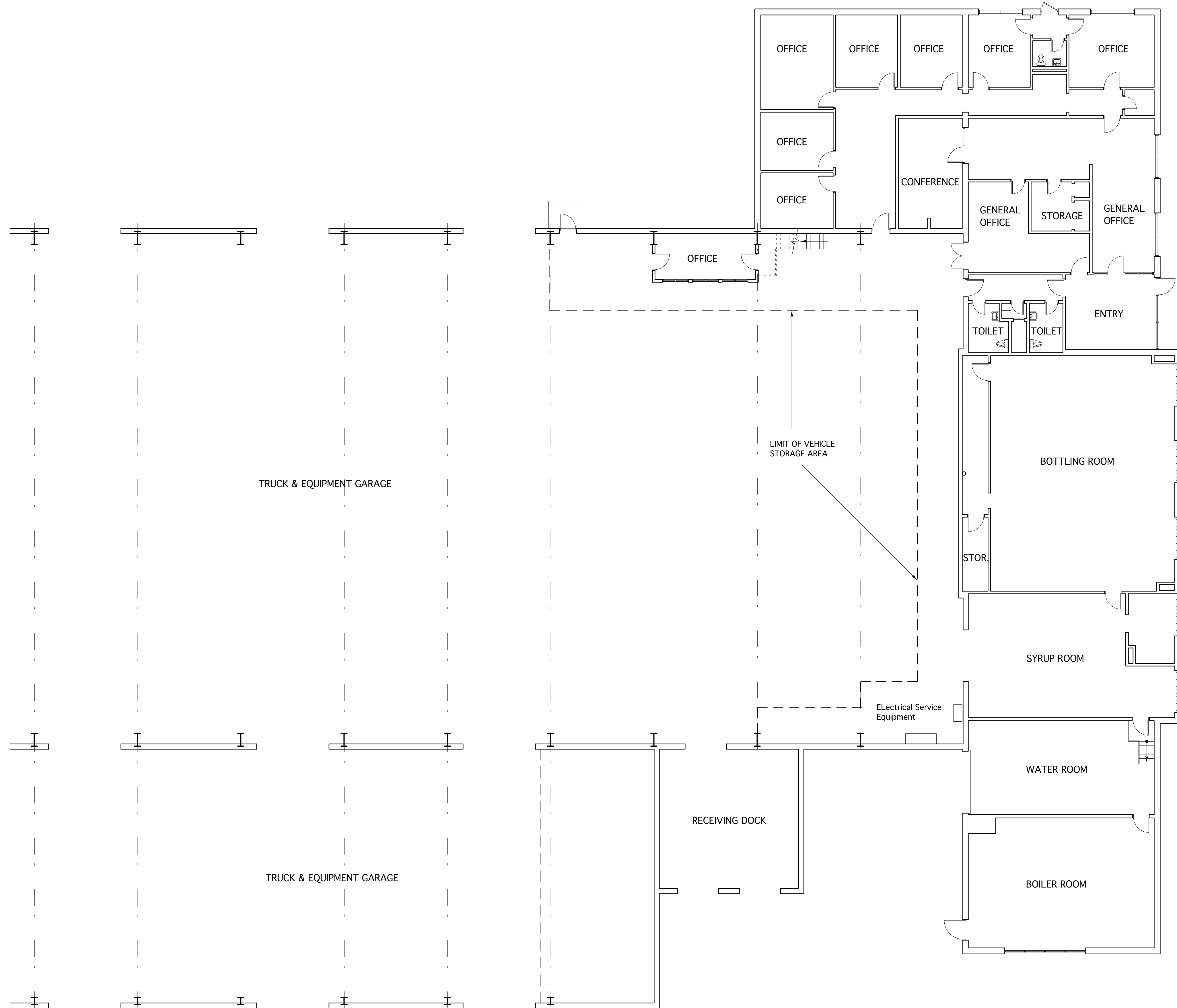
EXISTING CONDITIONS PLAN Scale: 3/32" = 1'-0"
