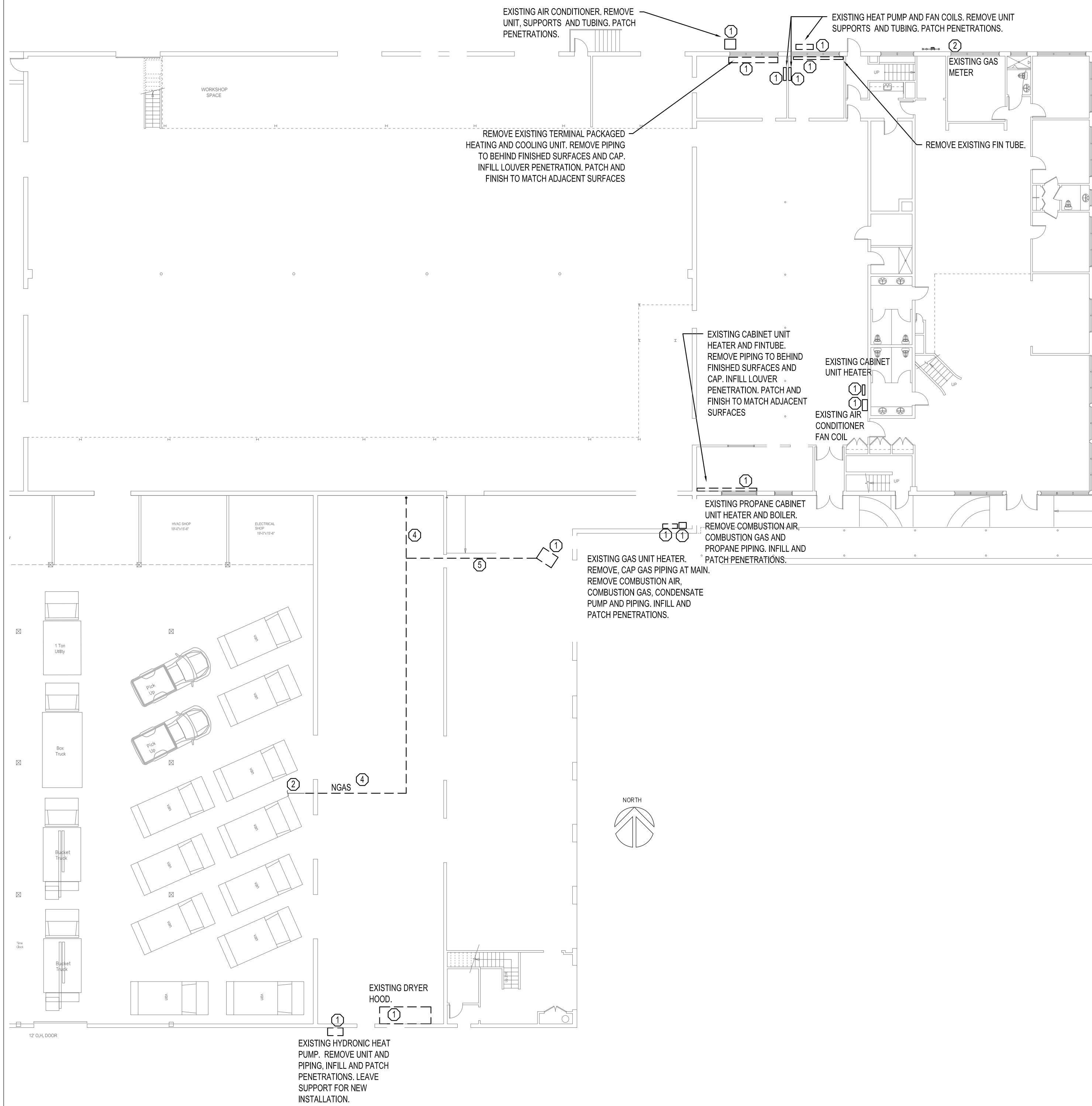
FIRST FLOOR HVAC PLAN - DEMOLITION SCALE: 1/16"=1'-0"
