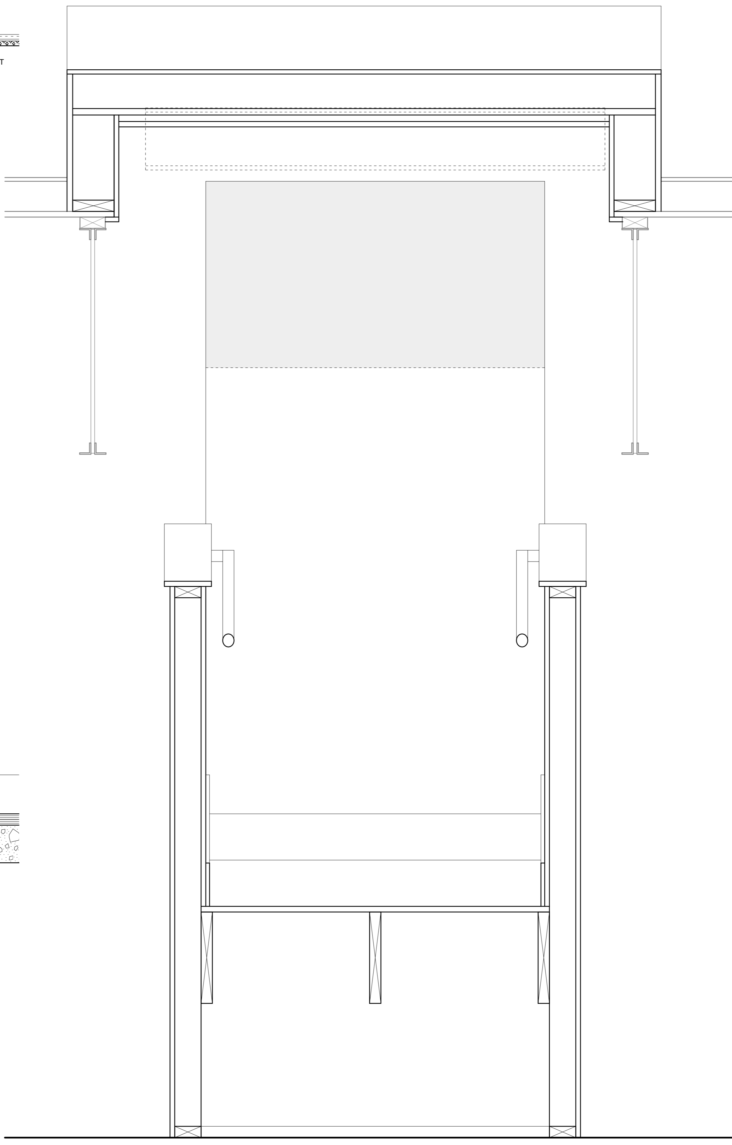
4 STAIR DETAIL SECTION SCALE: 1 1/2" = 1'-0"
