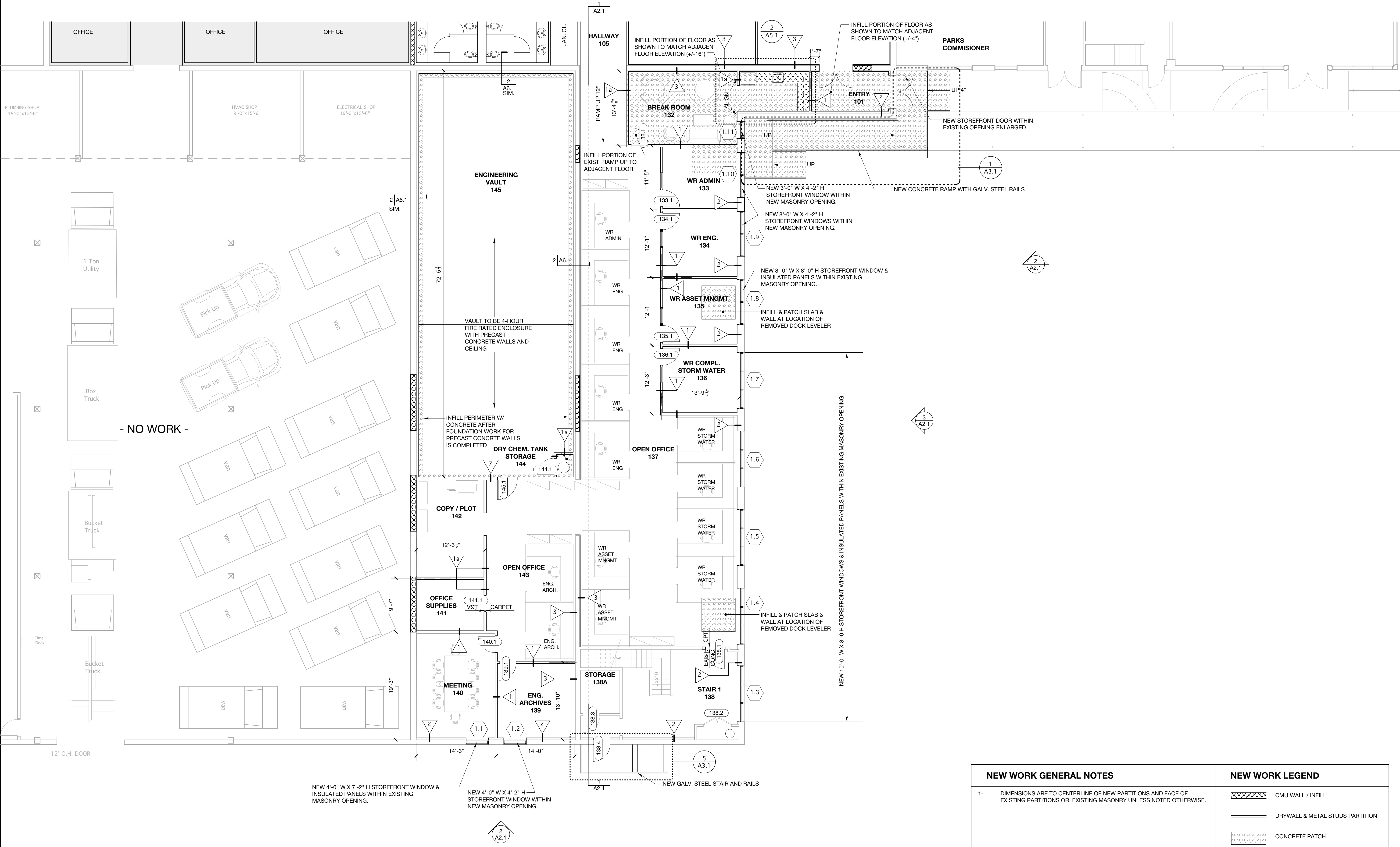
FIRST FLOOR PROPOSED PLAN - SOUTH SECTION 1/8" = 1'-0"
