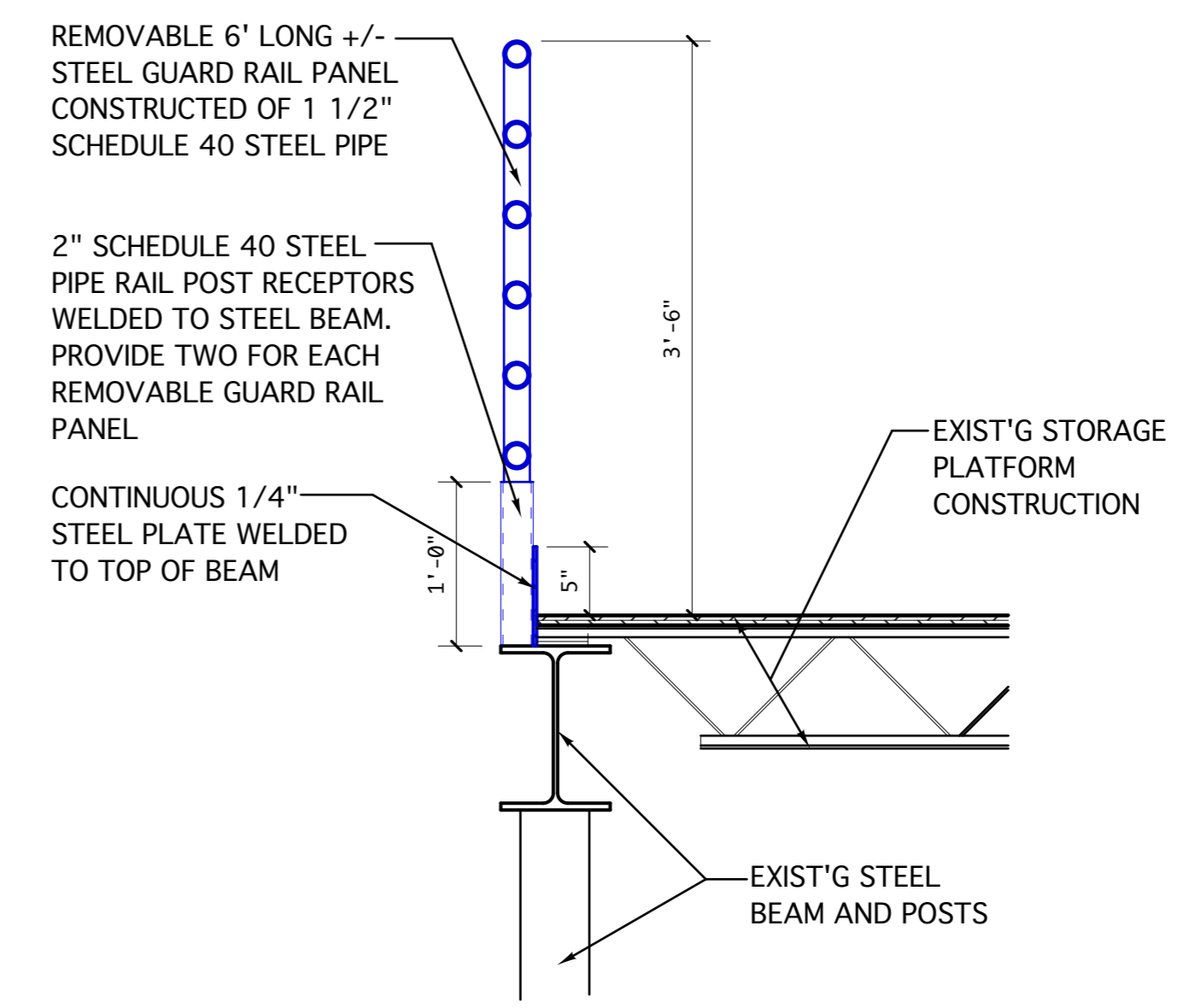
1 STORAGE PLATFORM REMOVABLE GUARD RAIL SECTION DETAIL 1" = 1'-0"
